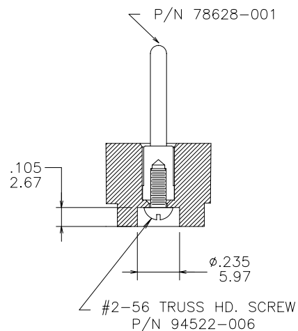
SECTION U-U
