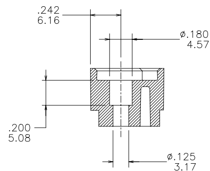
SECTION W-W
