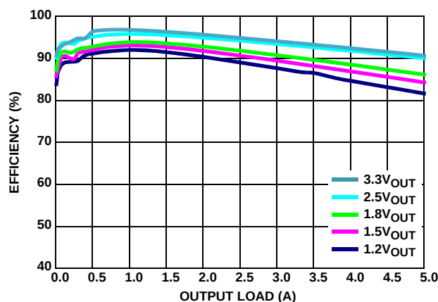
FIGURE 2. EFFICIENCY vs LOAD F SW = 1MHz, V IN = 5V, MODE = PFM, T A = +25 °C
