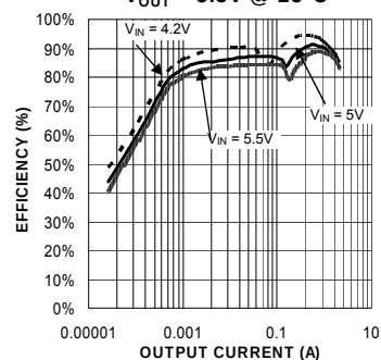
Efficiency vs. Output Current V_{OUT} = 3.3V @ 25^{\circ}C
