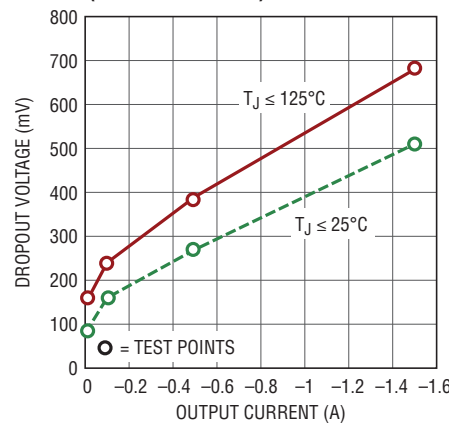
Guaranteed Dropout Voltage (DD-PAK/TQ-220)
