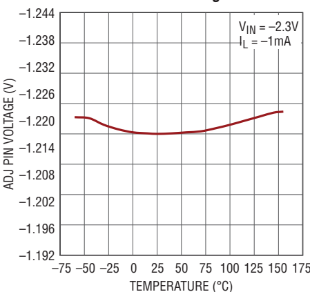
LT3015 ADJ Pin Voltage
