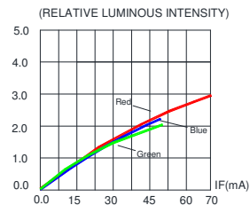
FIG.2 RELATIVE LUMINOUS INTENSITY VS. FORWARD CURRENT
