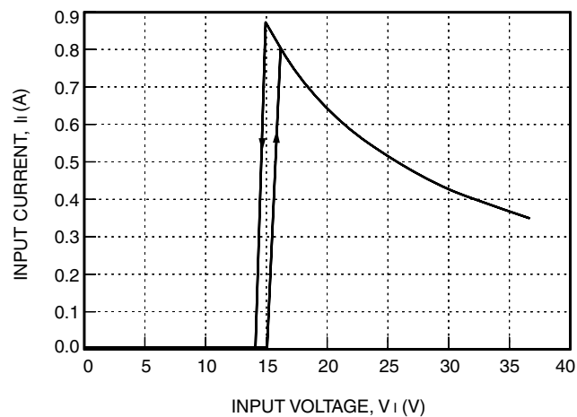
Figure 1. LC010 Input Current vs. Input Voltage at I_o = I_{o, \text{max}} and T_c = 25^\circ\text{C}
