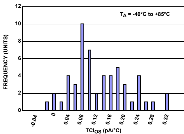
FIGURE 32. TCI_{OS} HISTOGRAM
