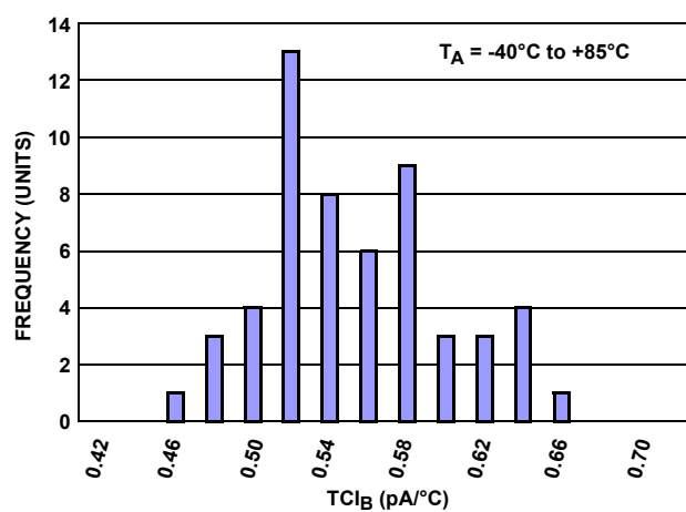
FIGURE 33. TCI_B HISTOGRAM
