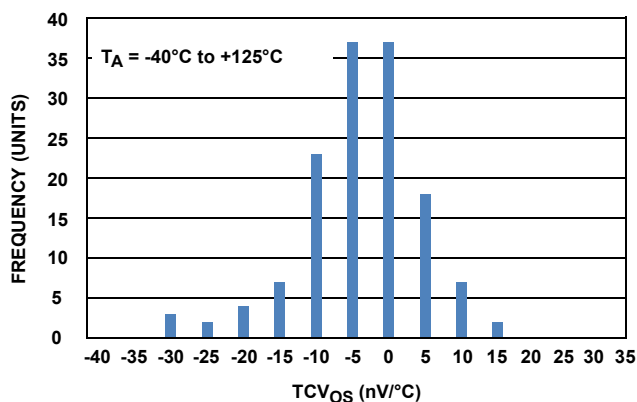
FIGURE 34. TCV_{OS} HISTOGRAM
