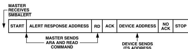
Figure 6. Use of \overline{\text{SMBALERT}}
