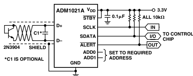
Figure 8. Typical Application Circuit
