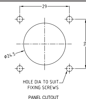
Cliffcon S 4 Pole Chassis Socket (Large Square Type) Compatible with all Cliffcon S 4 Pole Plugs Dimensions: 40 x 40 x 33mm
