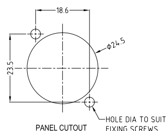
Cliffcon S 4 Pole Chassis Socket Compatible with all Cliffcon S 4 Pole Plugs Dimensions: 24 x 24 x 33mm
