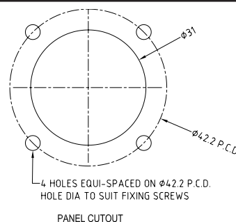
Cliffcon S 4 Pole Chassis Socket (Round Type) Compatible with all Cliffcon S 4 Pole Plugs Dimensions: 50 x 50 x 33mm
