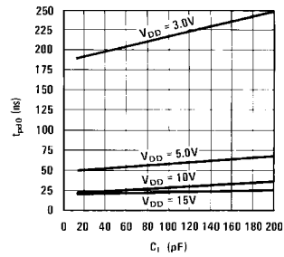
Typical Propagation Delay to a Logical "0" for the MM74C902
