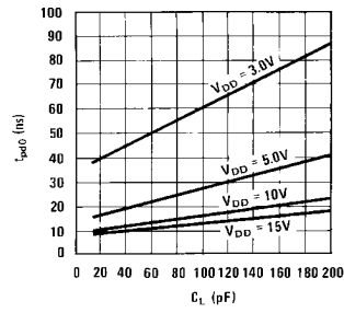
Typical Propagation Delay to a Logical "0" for the MM74C901
