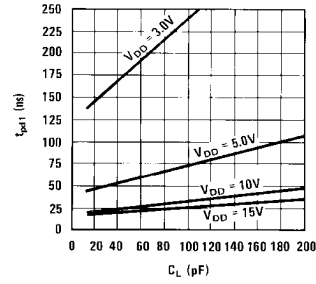
Typical Propagation Delay to a Logical "1" for the MM74C902
