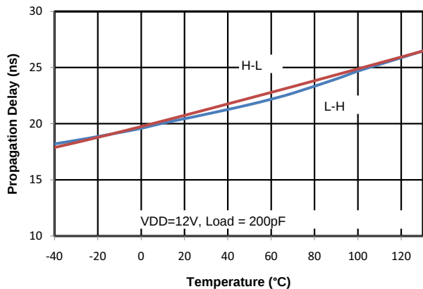
Figure 27. Propagation Delay vs. Temperature
