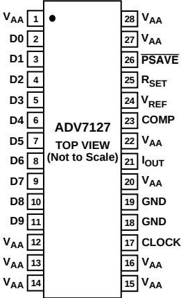
28-Lead SOIC
