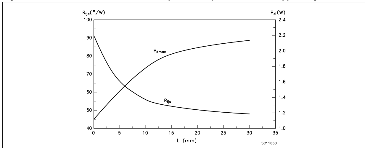
Figure 7. Thermal resistance &amp; maximum power dissipation vs P.C.B. copper length for DPAK
