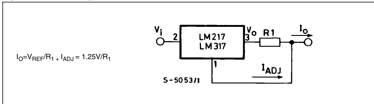
Figure 10. Current regulator
