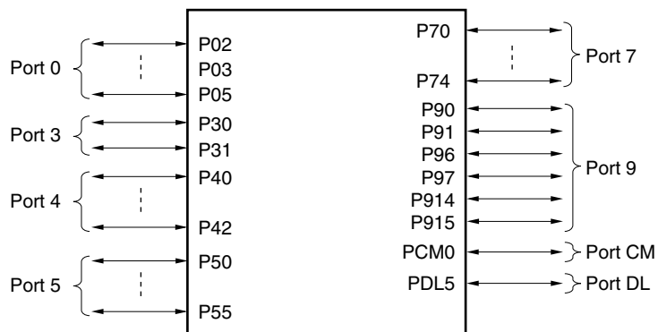
Figure 4-1. Port Configuration (V850ES/JC3-L (40-pin))
