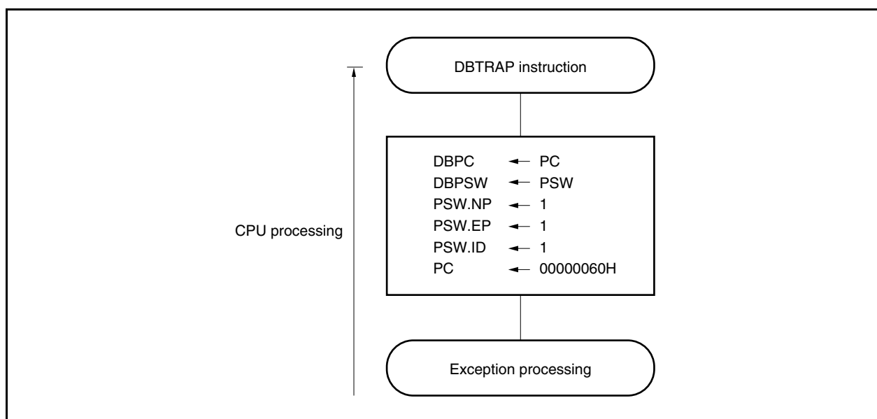
Figure 19-13. Debug Trap Processing
