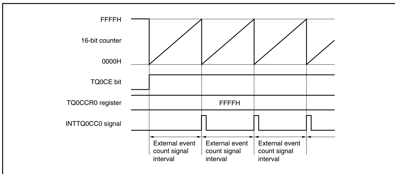
Figure 7-21. Operation When TQ0CCR0 Register Is Set to FFFFH
