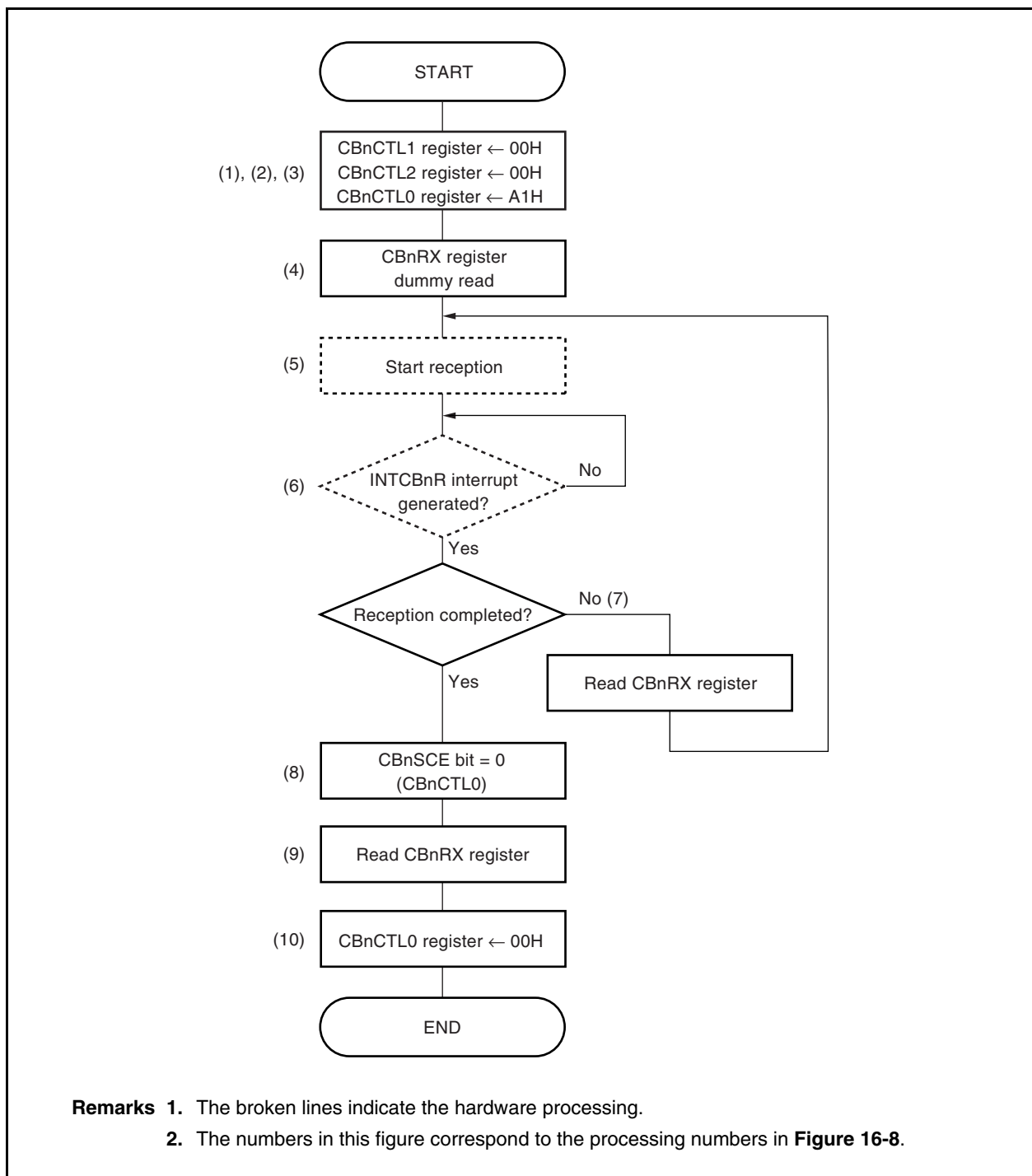
Figure 16-7. Single Transfer Mode Operation (Master Mode, Reception Mode)
