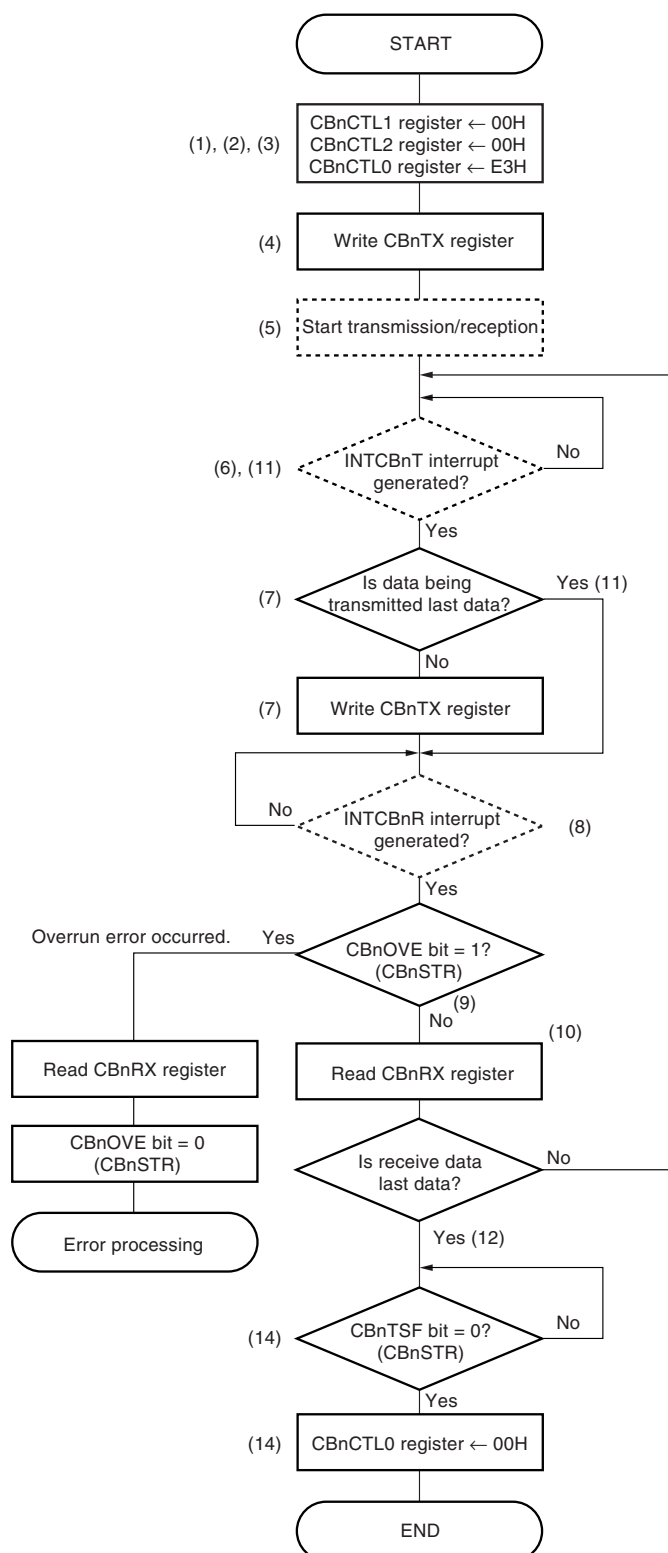
Figure 16-21. Continuous Transfer Mode Operation (Master Mode, Transmission/Reception Mode)
