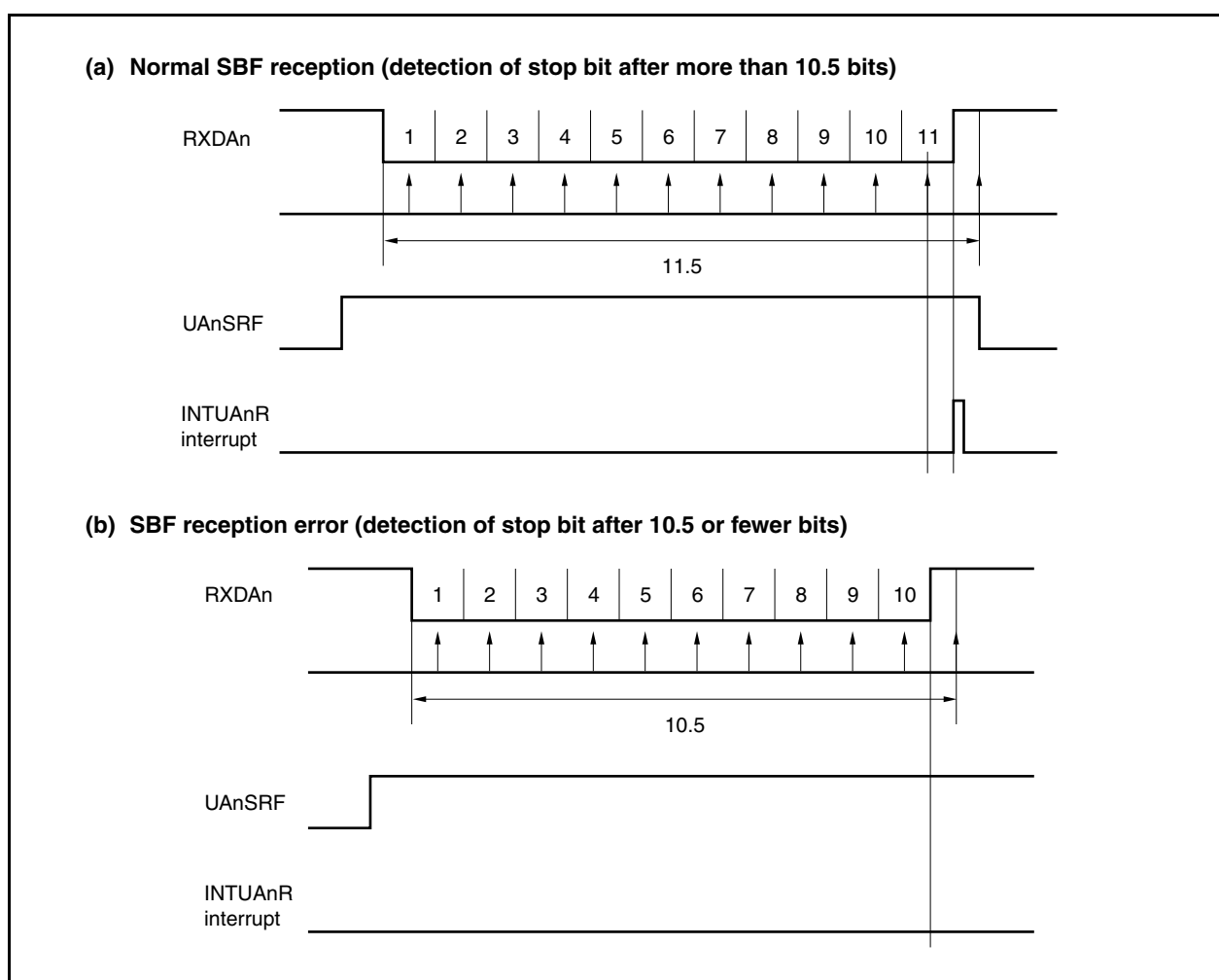
Figure 15-14. SBF Reception
