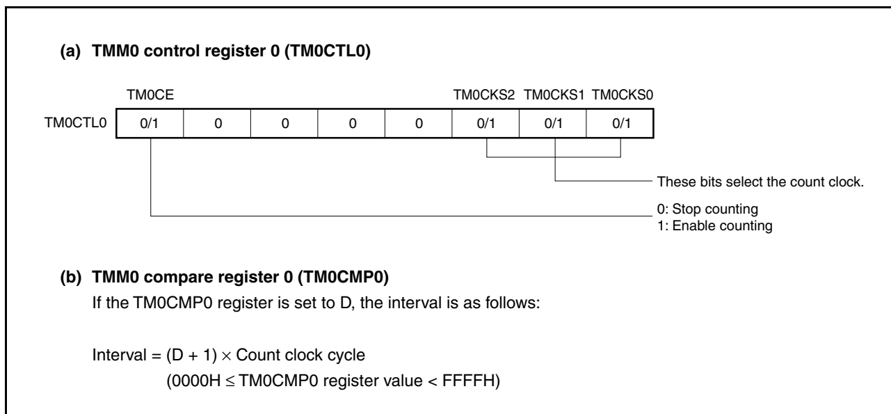
Figure 8-4. Register Settings in Interval Timer Mode
