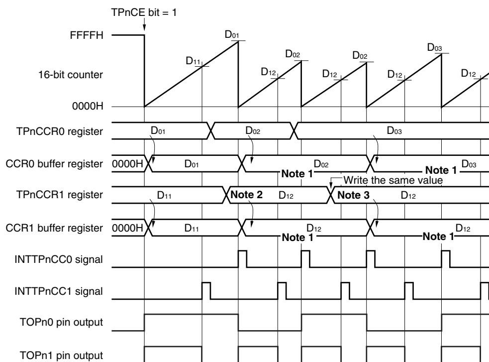
Figure 6-5. Batch Write Timing
