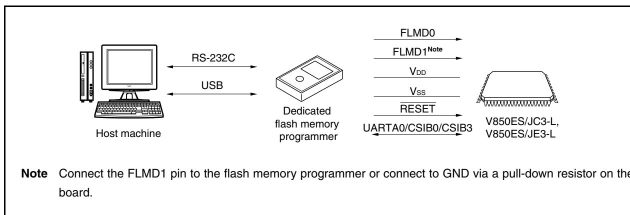
Figure 28-2. Environment Required for Writing Programs to Flash Memory
