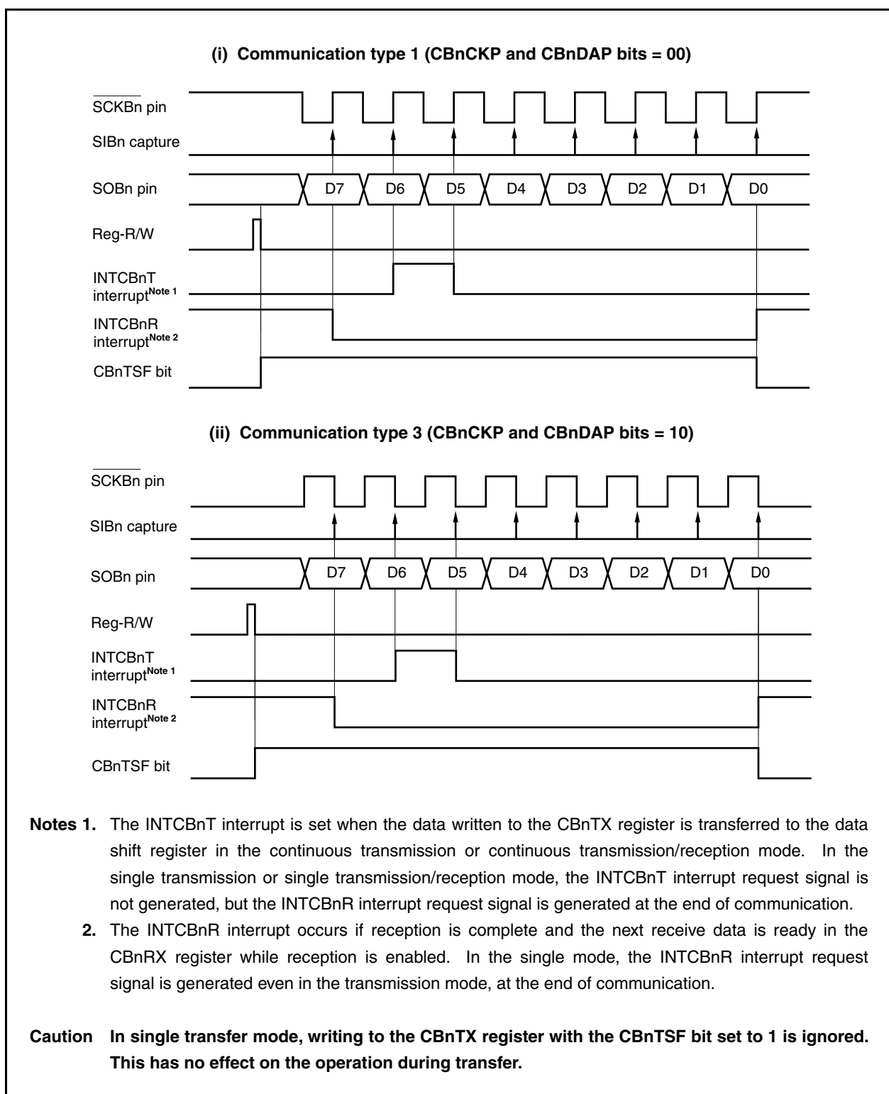
Figure 16-30. Clock Timing (1/2)
