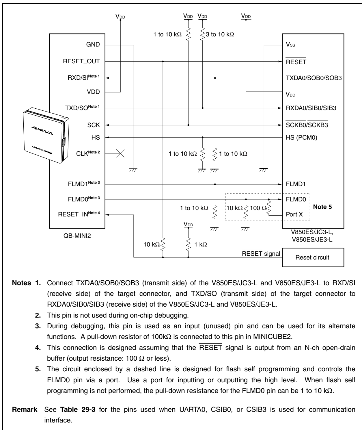
Figure 29-4. Circuit Connection Example When UARTA0/CSIB0/CSIB3 Is Used for Communication Interface
