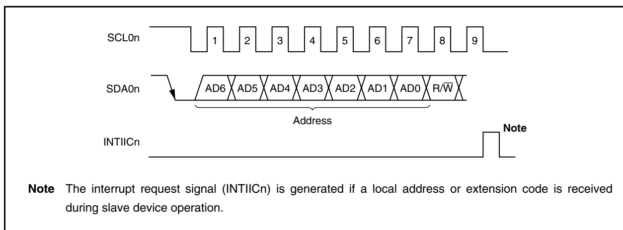
Figure 17-9. Address
