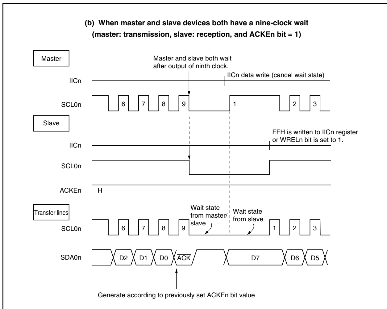
Figure 17-13. Wait State (2/2)
