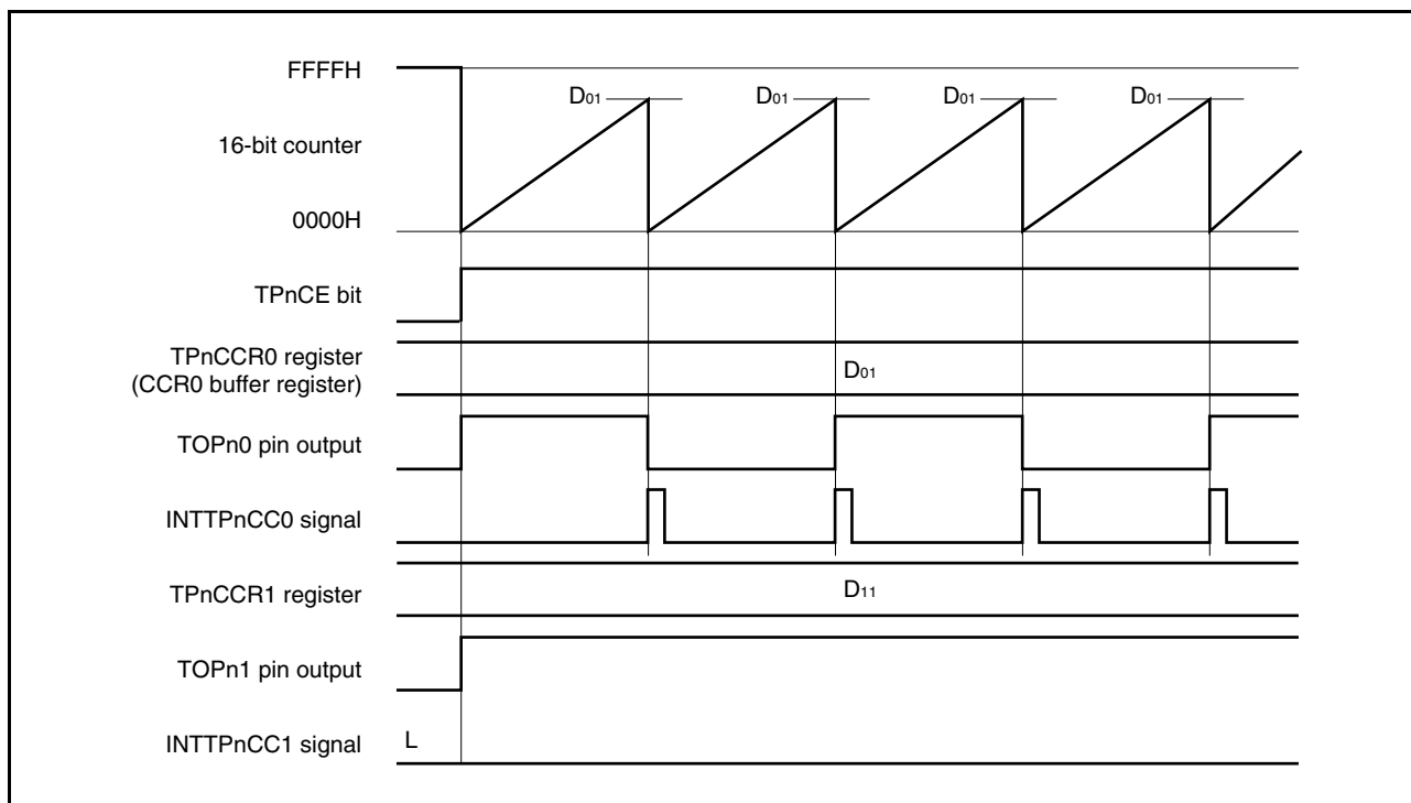
Figure 6-15. Timing of Operations When D_{01} < D_{11}
