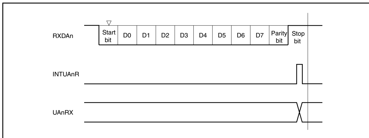
Figure 15-9. UART Reception
