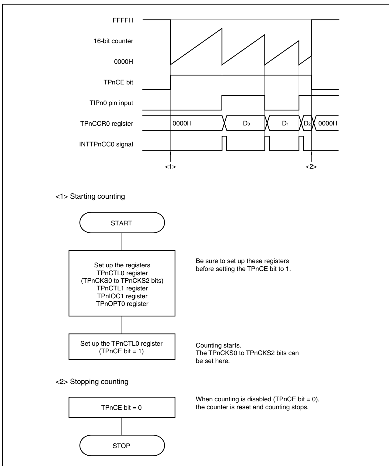
Figure 6-68. Timing and Processing of Operations in Pulse Width Measurement Mode
