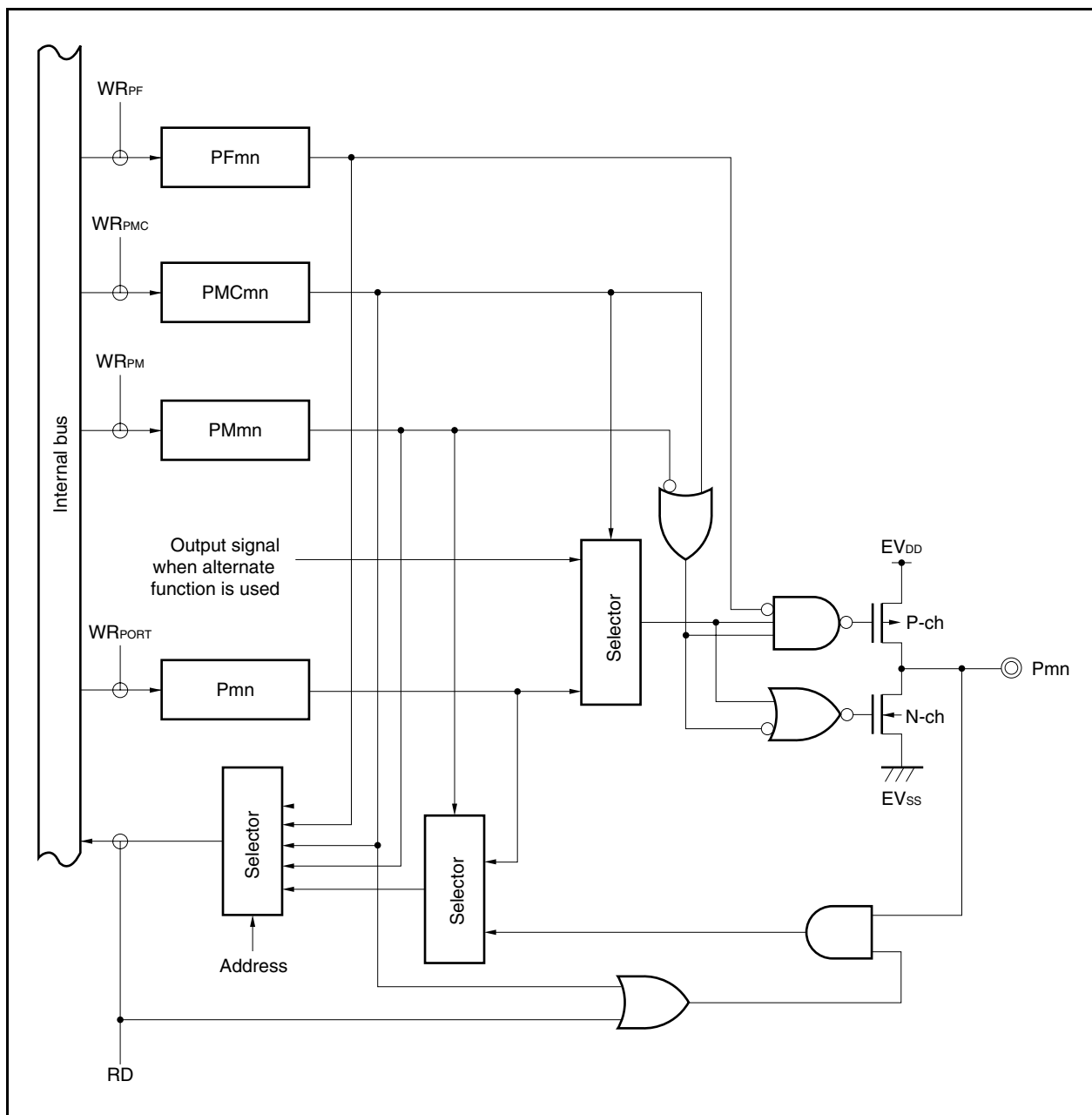
Figure 4-13. Block Diagram of Type G-13
