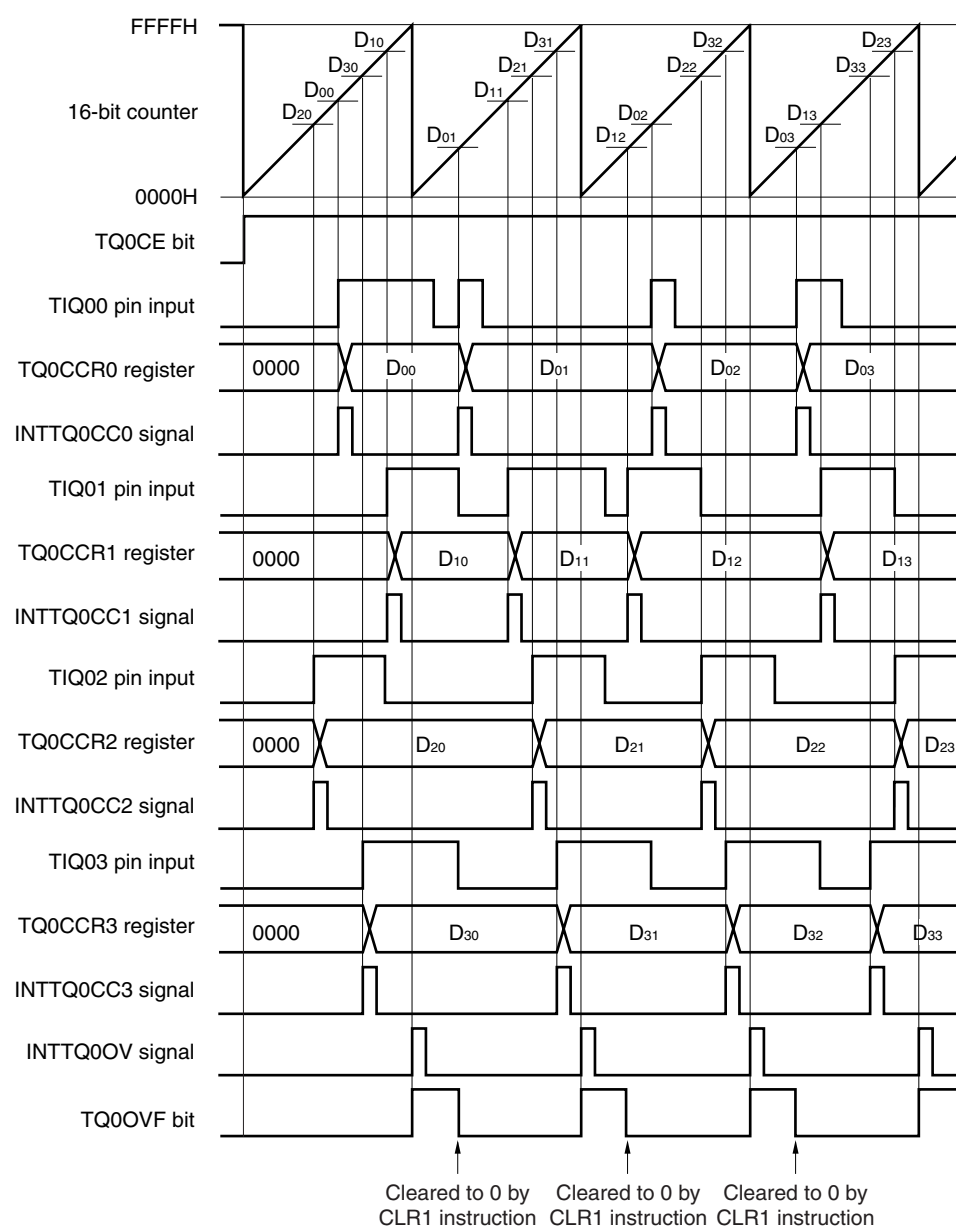
Figure 7-54. Basic Timing of Operations in Free-Running Timer Mode (Capture Function)
