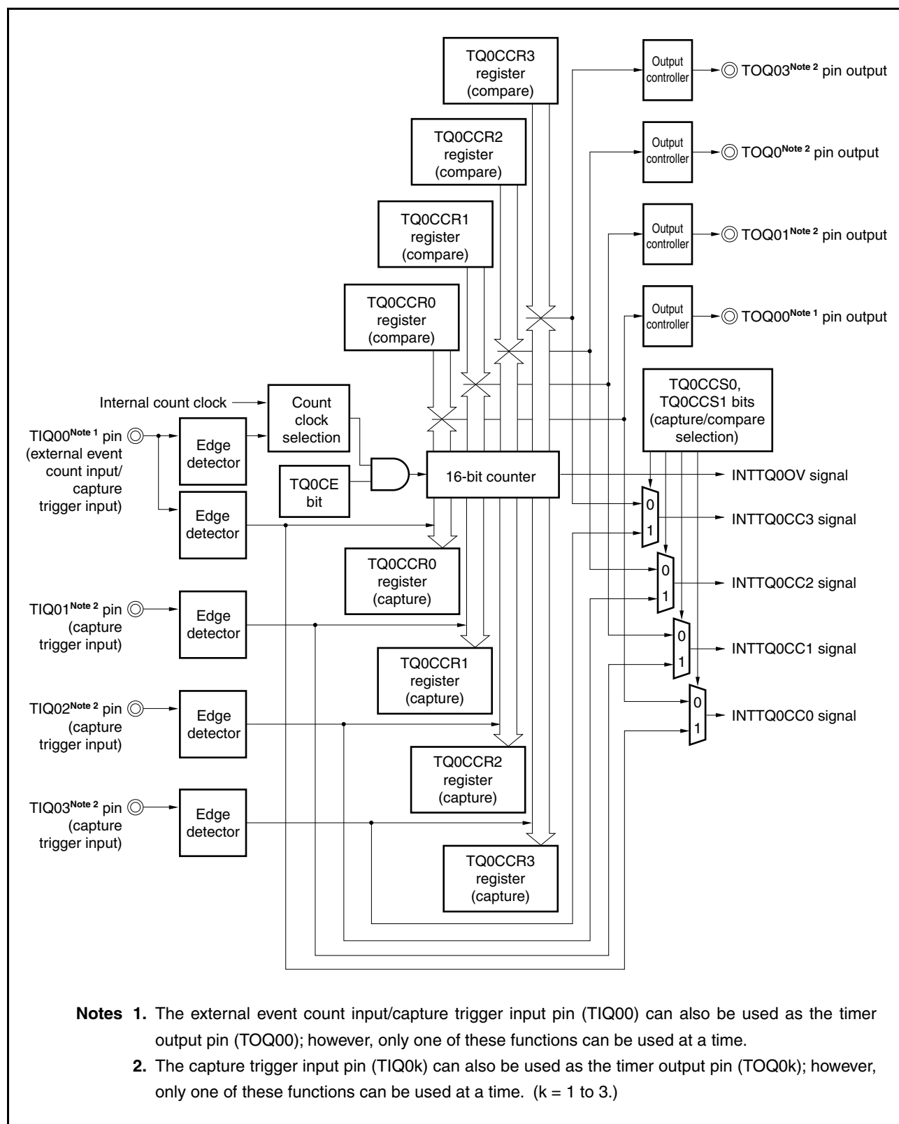
Figure 7-52. Configuration of TMQ0 in Free-Running Timer Mode
