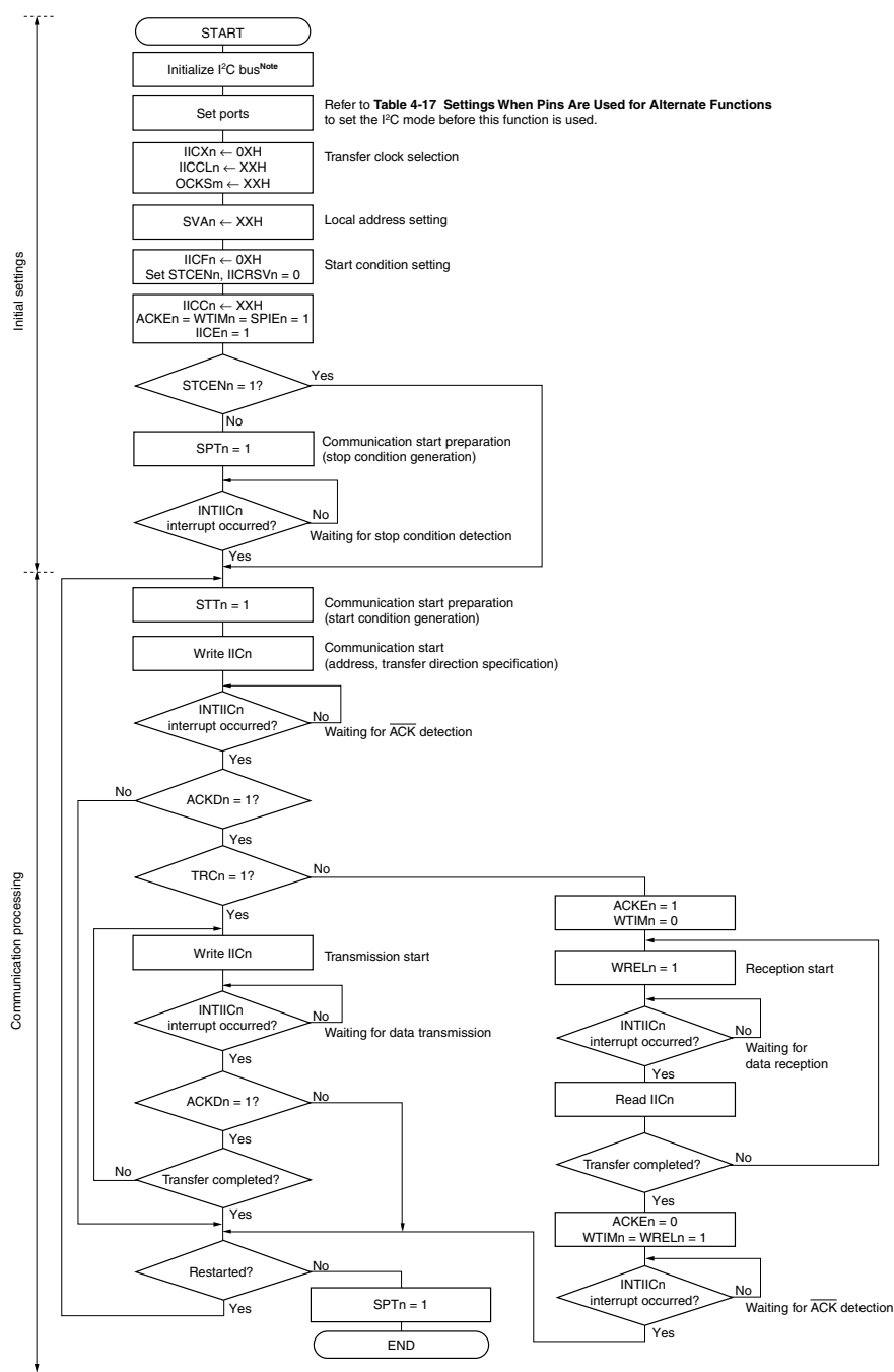
Figure 17-18. Master Operation in Single Master System
