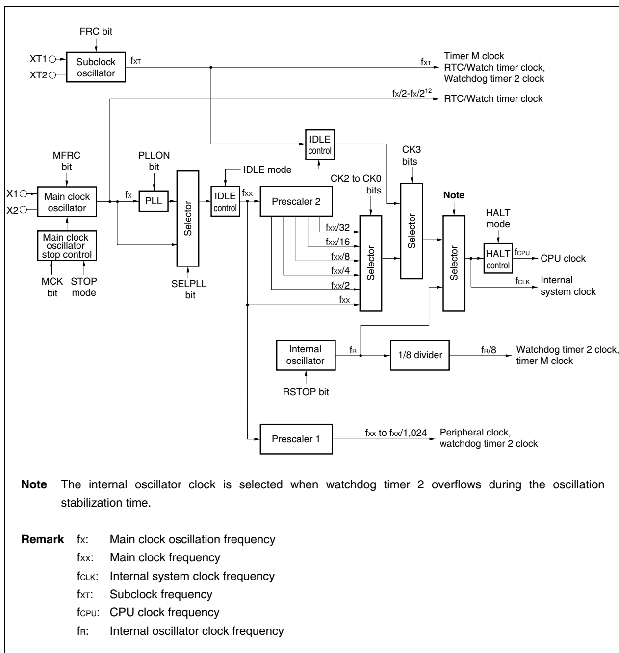
Figure 5-1. Clock Generator
