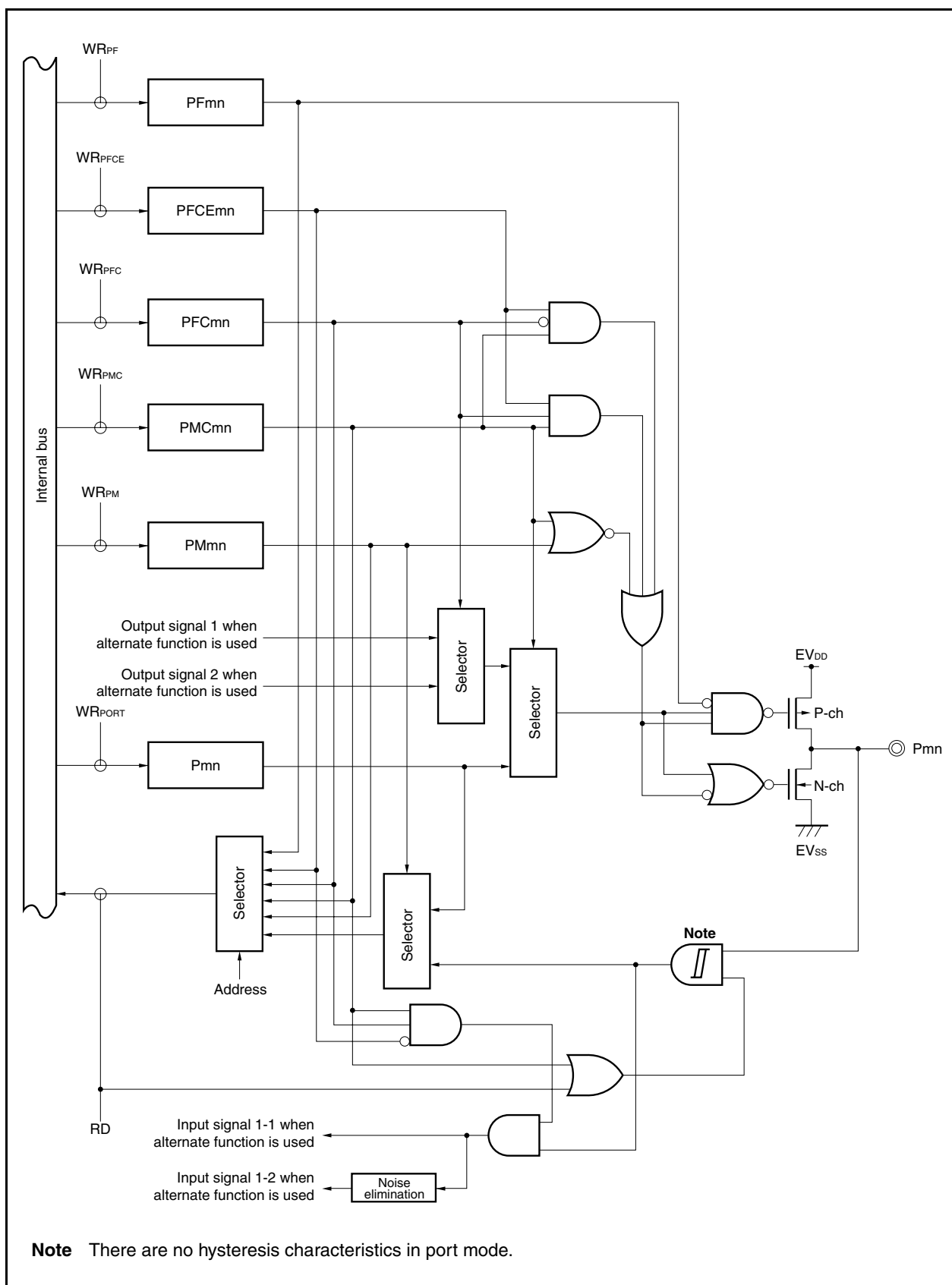
Figure 4-23. Block Diagram of Type U-5
