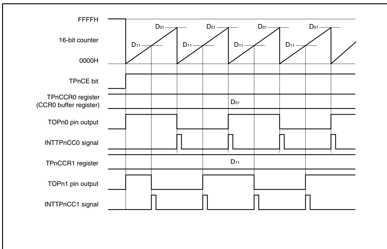
Figure 6-14. Timing of Operations When D_{01} \geq D_{11}
