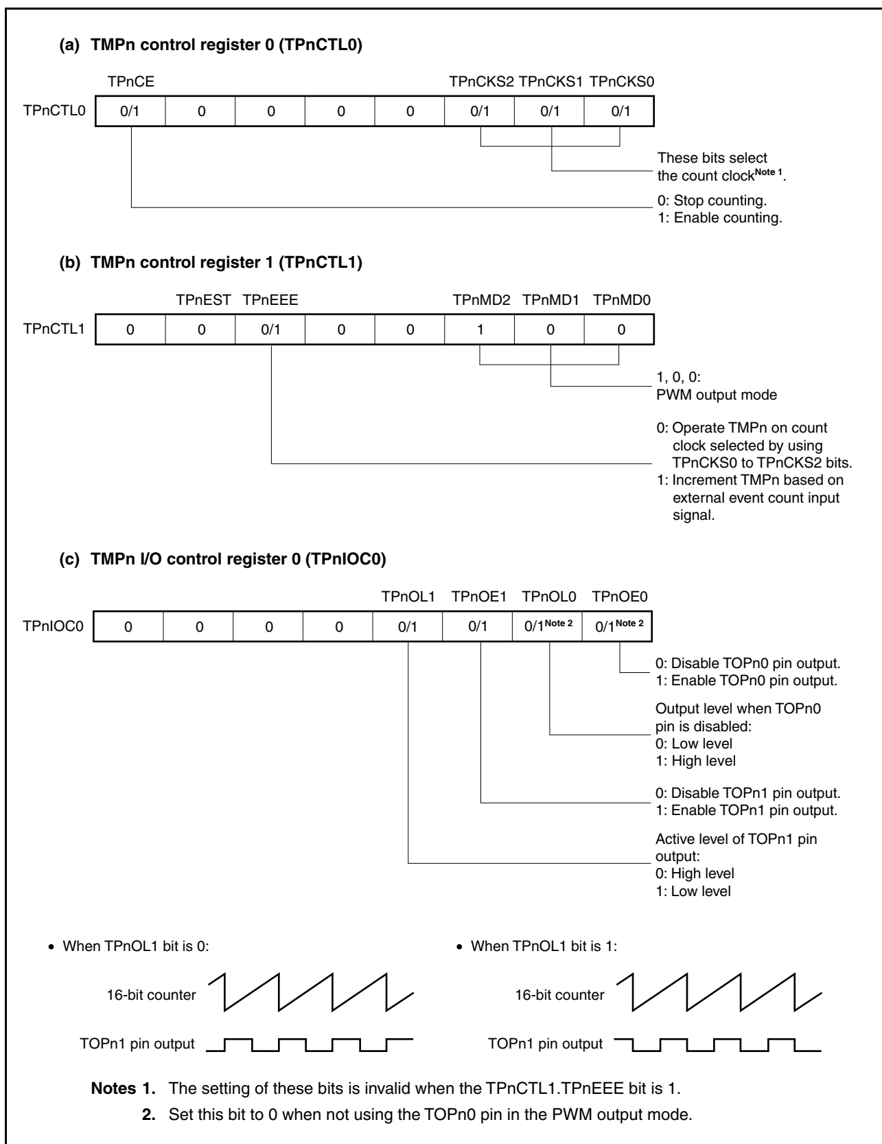
Figure 6-46. Register Settings in PWM Output Mode (1/2)
