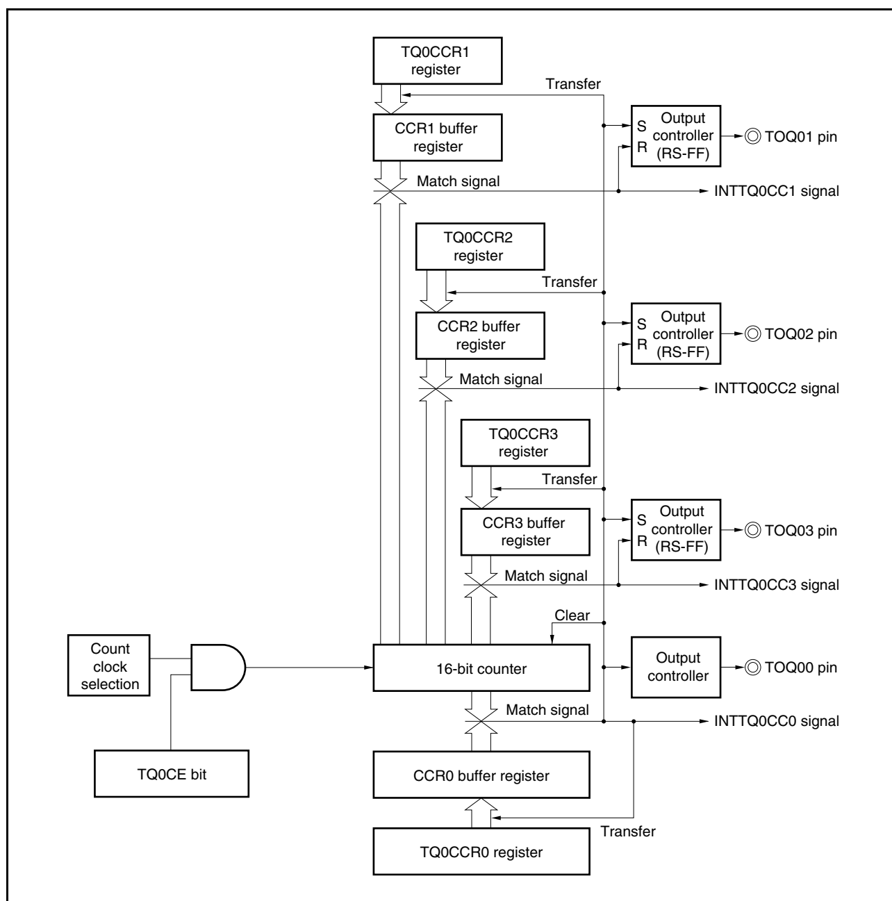
Figure 7-44. Configuration of TMQ0 in PWM Output Mode
