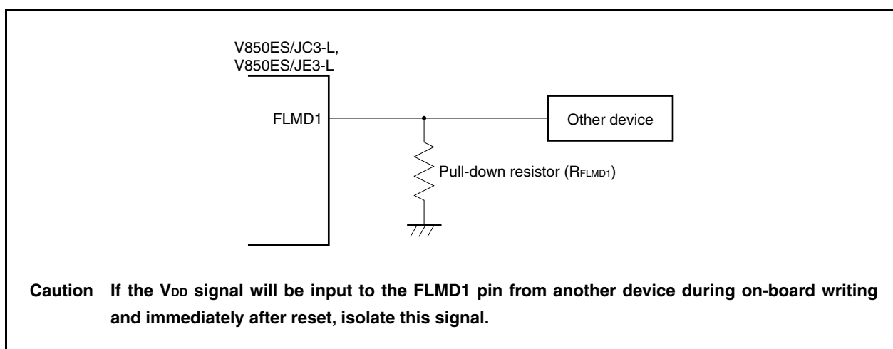
Figure 28-10. FLMD1 Pin Connection Example
