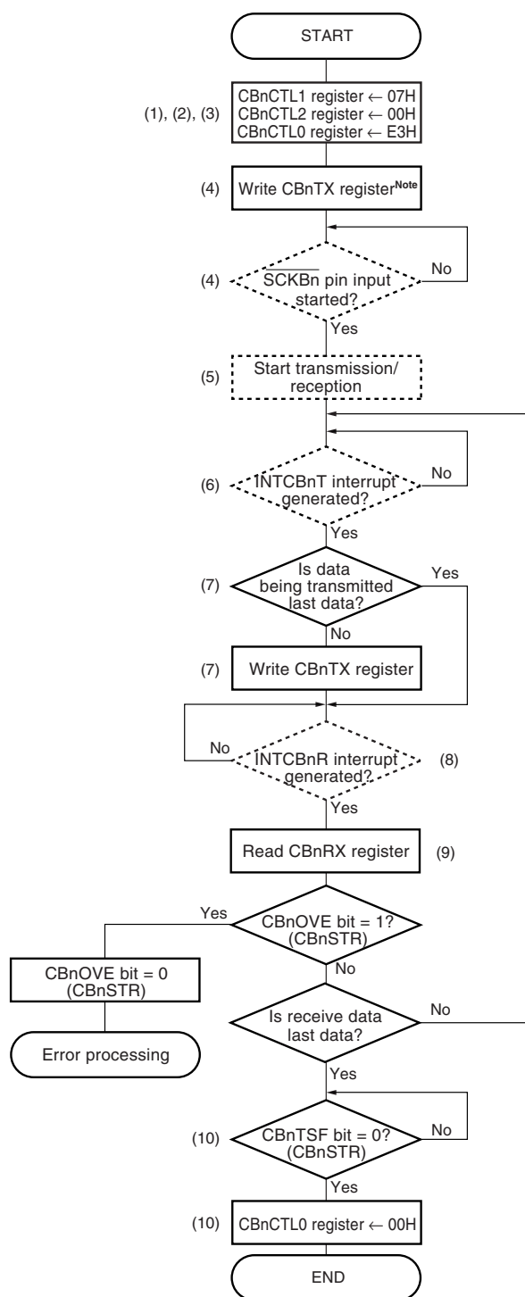
Figure 16-27. Continuous Transfer Mode Operation (Slave Mode, Transmission/Reception Mode)
