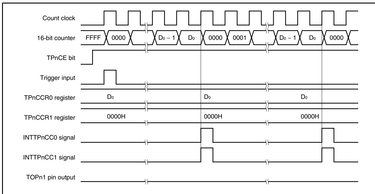
Figure 6-31. Outputting 0% PWM Waveform
