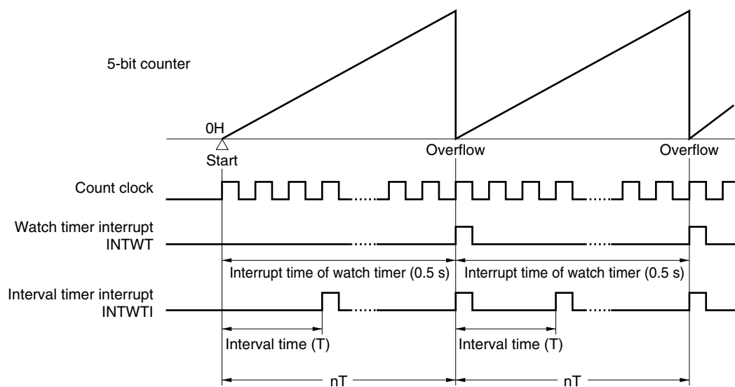
Figure 9-2. Timing of Watch Timer and Interval Timer Operations
