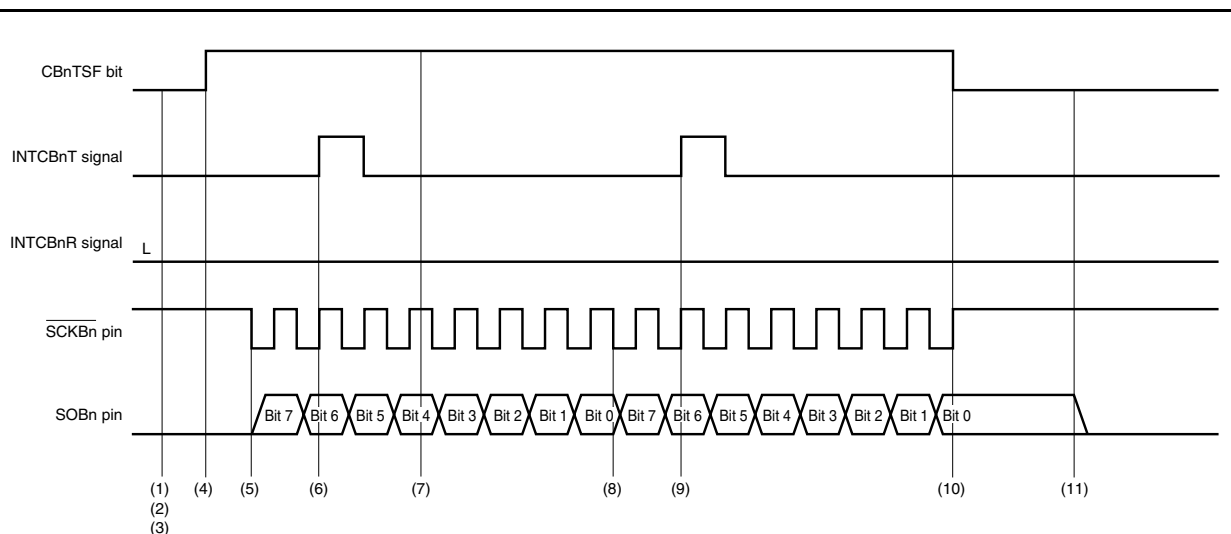
Figure 16-18. Continuous Transfer Mode Operation Timing (Master Mode, Transmission Mode)
