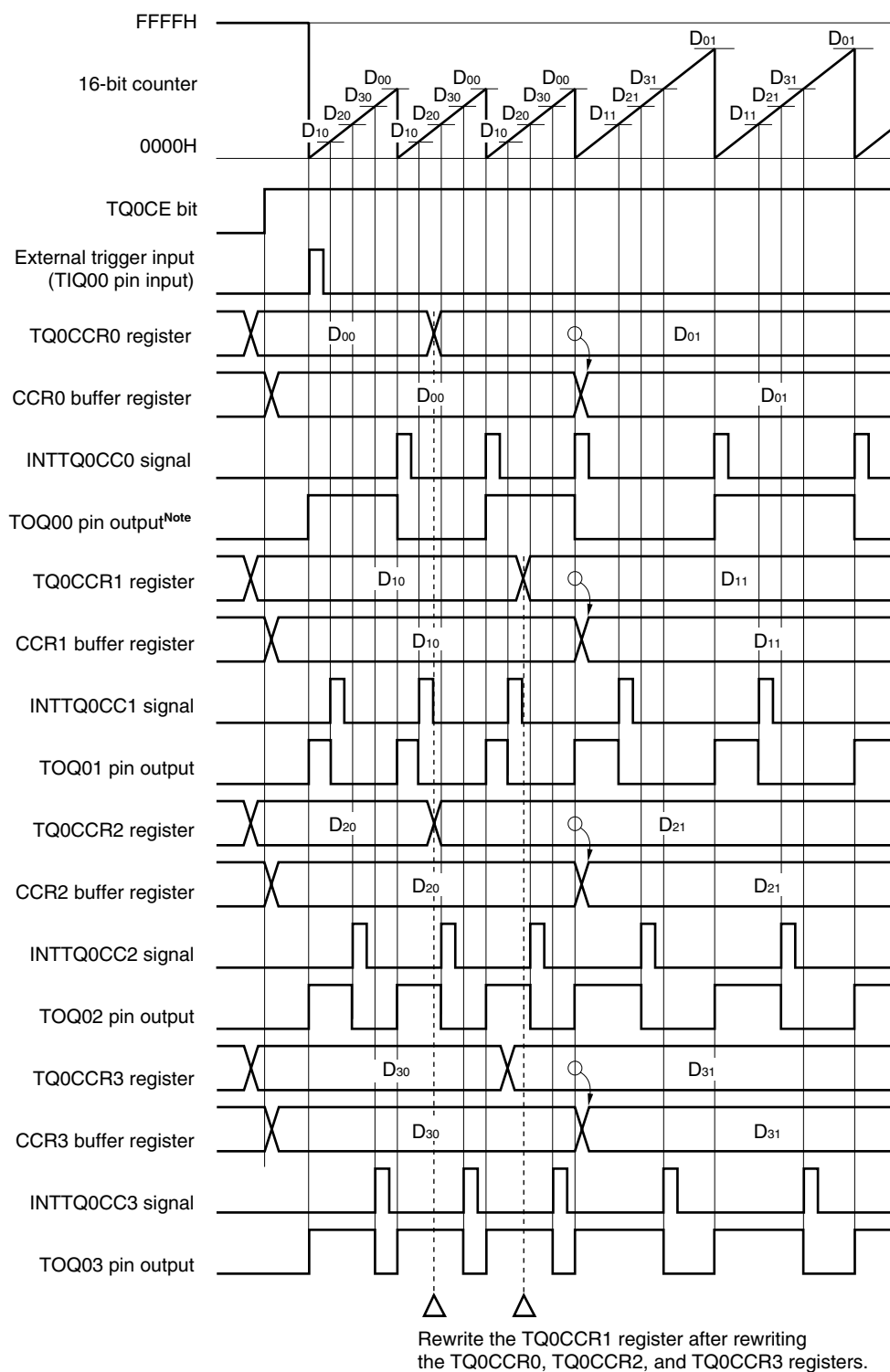
Figure 7-30. Changing PWM Waveform While Counter Is Incrementing
