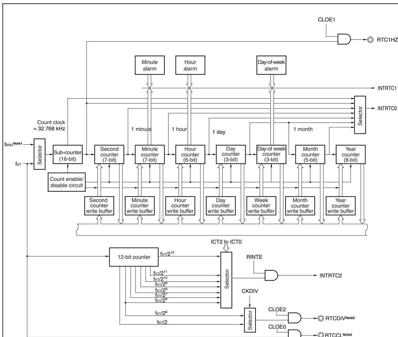
Figure 10-1. Block Diagram of Real-Time Counter
