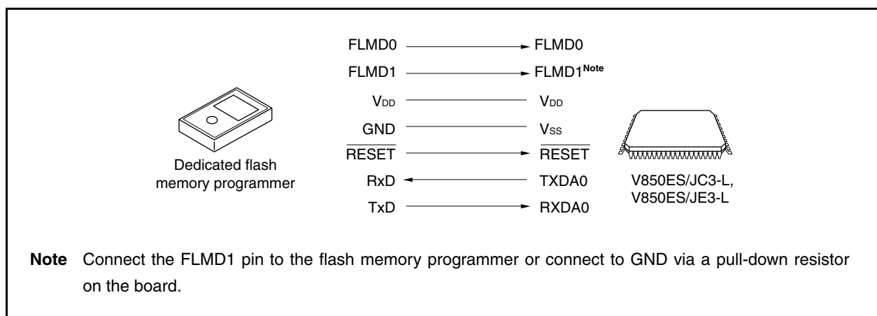
Figure 28-3. Communication with Dedicated Flash Memory Programmer (UARTA0)
