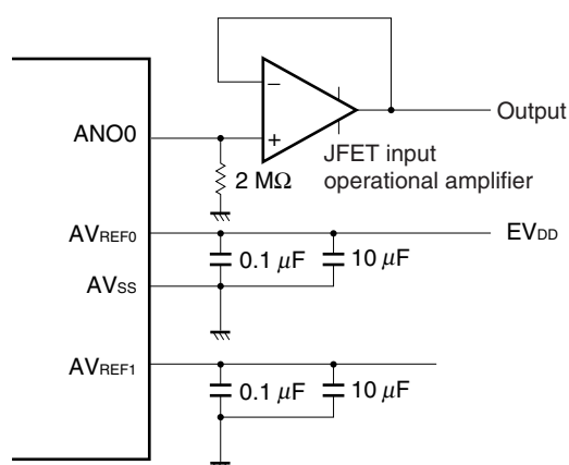
Figure 14-2. Example of External Pin Connection
