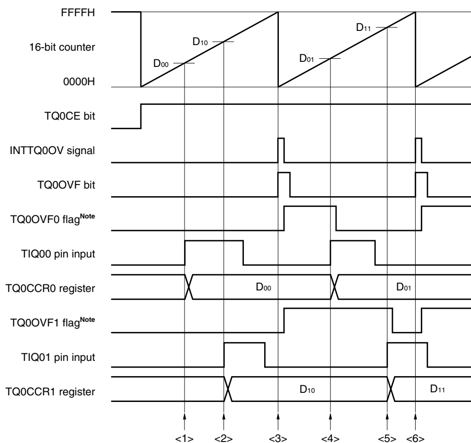
Figure 7-61. Example of Resolving Problem When Two or More Capture Registers Are Used by Using Overflow Interrupt
