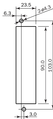
Direct Mounting Strip FC4A-PSP1P
