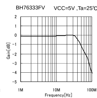
Fig.80 Frequency Response
