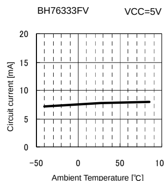
Fig.64 ICC1 vs. Ambient Temperature
