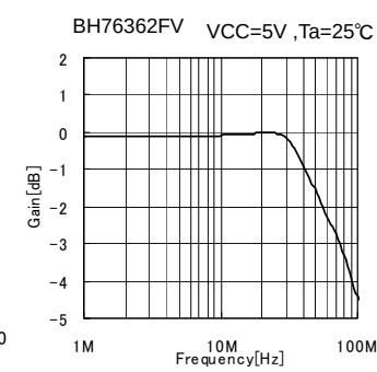
Fig.79 Frequency Response
