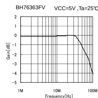
Fig.80 Frequency Response
