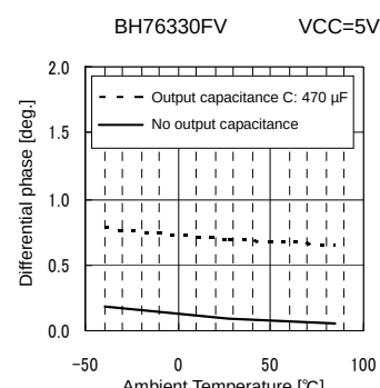
Fig.52 DP vs. Ambient Temperature
