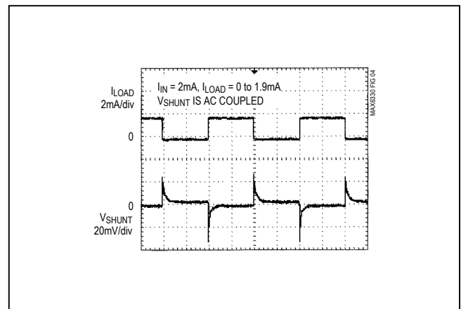
Figure 4. Load-Transient Response with C L = 0.0047 \mu F
