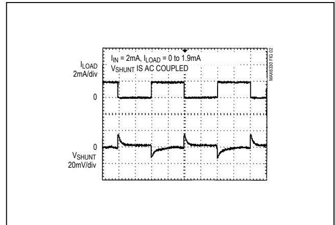
Figure 2. Load-Transient Response with C L = 0.22 \mu F
