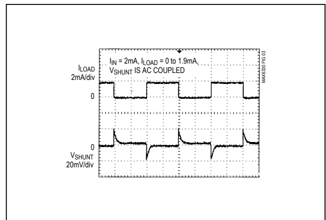
Figure 3. Load-Transient Response with C L = 0.033 \mu F
