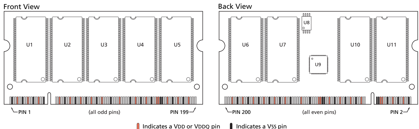
Figure 1: Module Layout
