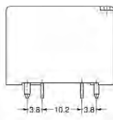
Terminal Arrangement/Internal Connections (Bottom View)
