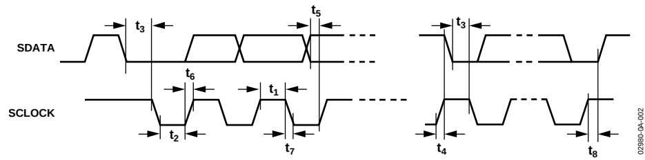
Figure 2. MPU Port Timing Diagram
