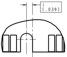
DETAIL B SCALE 8:1
