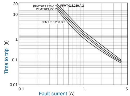
Typical Time to Trip at 23 °C
