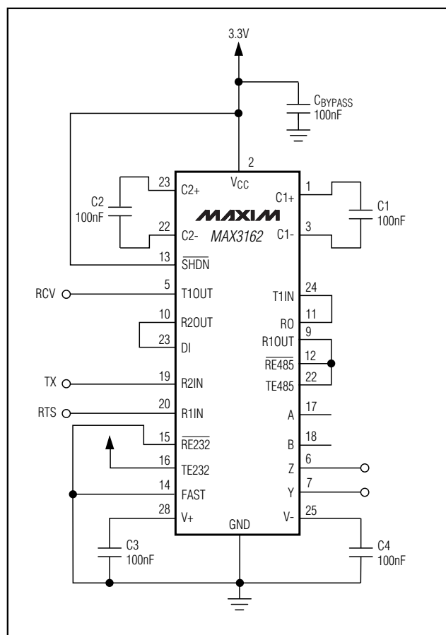
Figure 15. Protocol Translator
