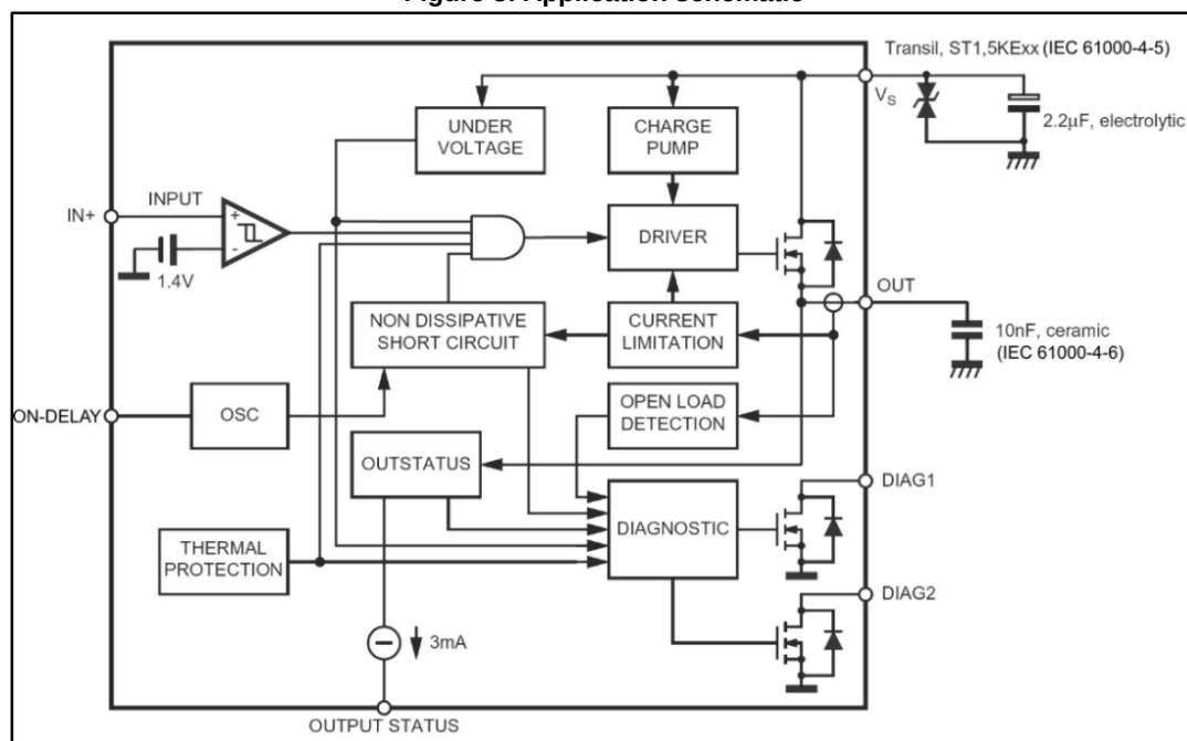
Figure 8: Application schematic
