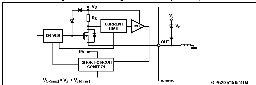
Figure 7: External demagnetization circuit (versus VS)
