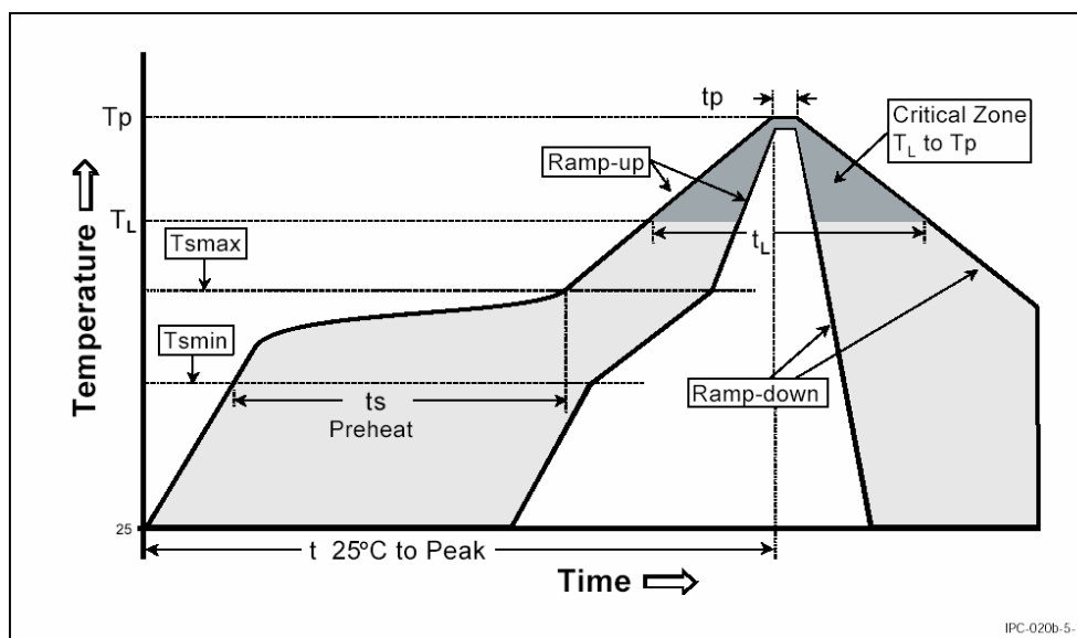
Figure 16. Recommended SCA100T body temperature profile during reflow soldering. Ref. IPC/JEDEC J-STD-020B.
