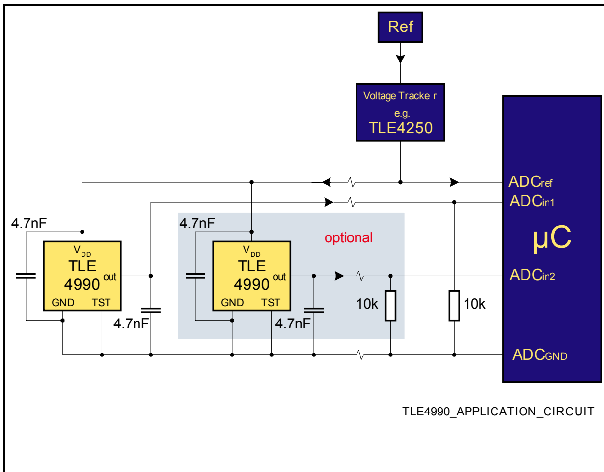
Figure 6 Application Circuit
