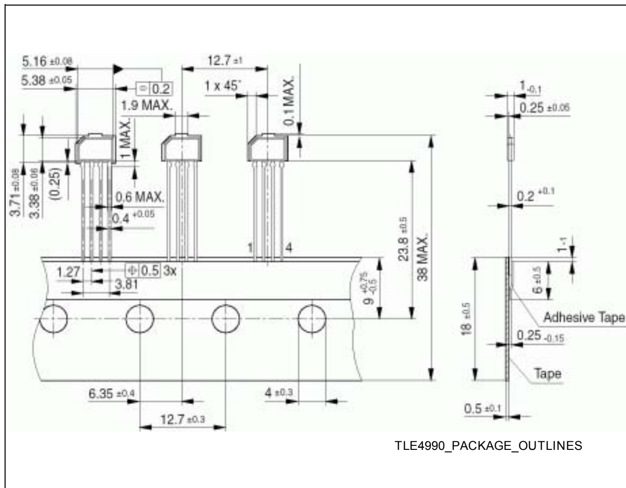
Figure 7 Package Outline
