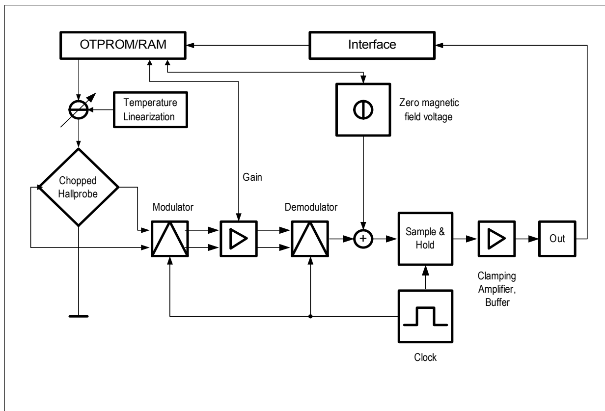
Figure 2 Block Diagram
