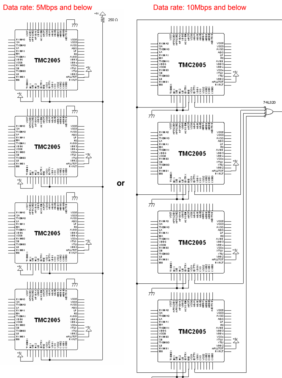
FIGURE 8 - APPLICATION EXAMPLE 8
