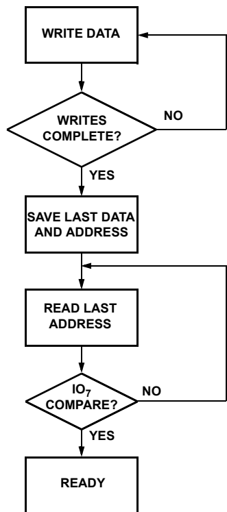
FIGURE 4. \overline{\text{DATA}} POLLING SOFTWARE FLOW
