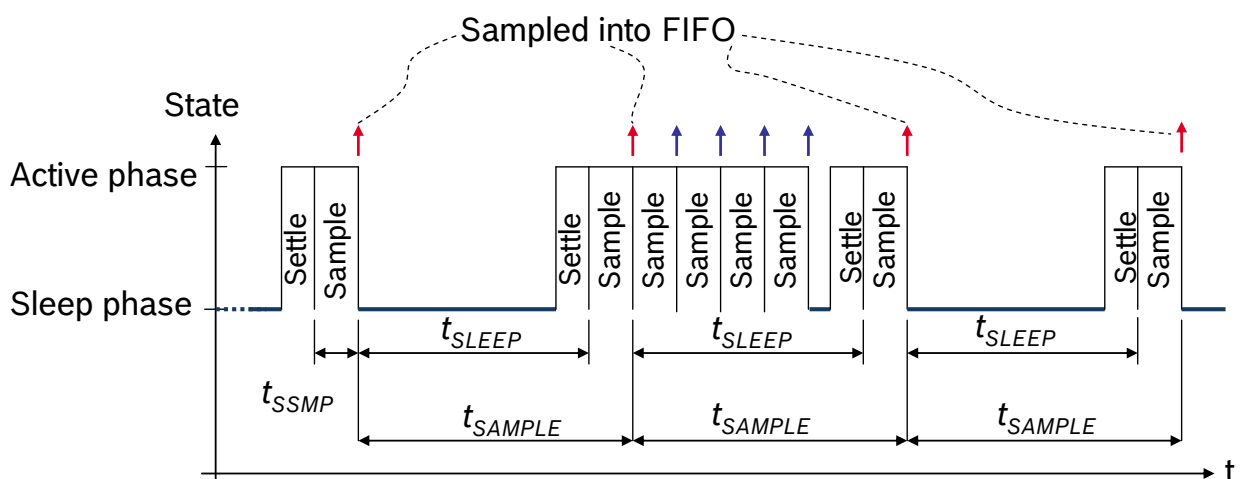
When (0x12) sleep_timer_mode is set to '1', the equidistant-sampling mode (EST) is selected. The use of the EST mode is recommended when the FIFO is used since it ensures that equidistant samples are sampled into the FIFO regardless of whether the active phase is extended by active interrupt engines or interface activity. In EST mode the sleep time t_{SLEEP,a} is defined as shown in Figure 4. The FIFO sampling time t_{SAMPLE,a} is the sum of the sleep time t_{SLEEP,a} and the sensor data sampling time t_{SSMP,a} . Since interrupt engines can extend the active phase to exceed the sleep time t_{SLEEP,a} , equidistant sampling is only guaranteed if the bandwidth has been chosen such that 1/(2 * bw) = n * t_{SLEEP,a} where n is an integer. If this condition is infringed, equidistant sampling is not possible. Once the sleep time has elapsed the device will store the next available sample in the FIFO. This set-up condition is not recommended as it may result in timing jitter.
