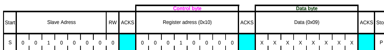
Figure 22: Example of an I 2 C write access
