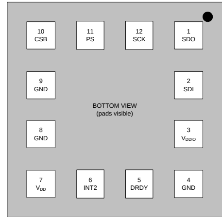
Figure 26: Pin-out bottom view
