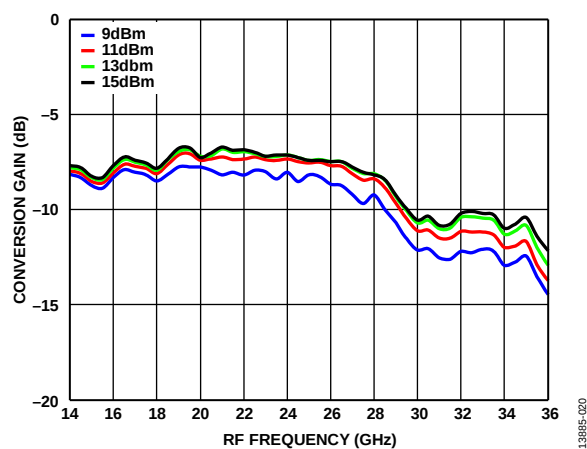
Figure 19. Conversion Gain vs. RF Frequency at Various LO Power Levels, T_A = 25^\circ\text{C}
