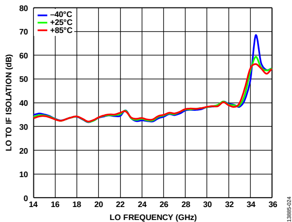
Figure 23. LO to IF Isolation vs. LO Frequency at Various Temperatures, LO = 13 dBm
