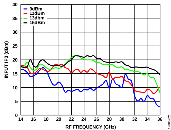
Figure 20. Input IP3 vs. RF Frequency at Various LO Power Levels, T_A = 25^\circ\text{C}
