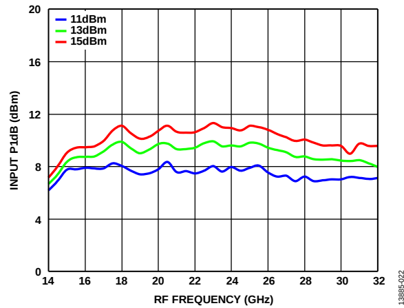
Figure 21. Input P1dB vs. RF Frequency at Various LO Power Levels, T_A = 25^\circ\text{C}
