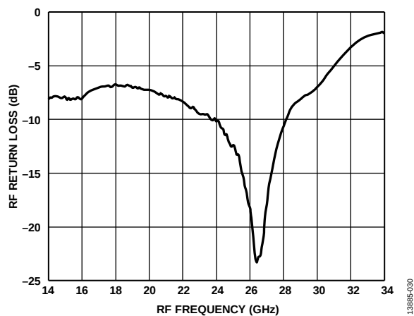
Figure 29. RF Return Loss vs. RF Frequency LO = 13 dBm at 17 GHz
