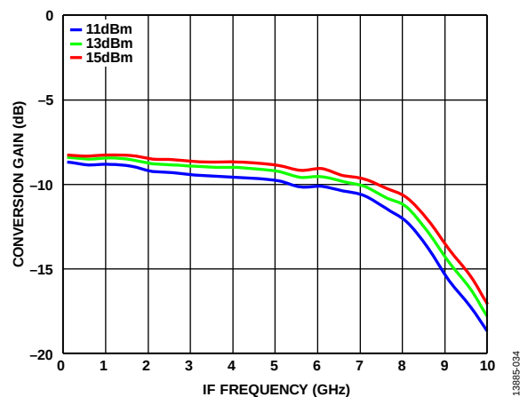
Figure 33. Conversion Gain vs. IF Frequency at Various LO Power Levels, T_A = 25^\circ\text{C}
