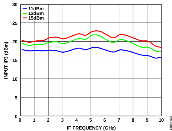
Figure 34. Input IP3 vs. IF Frequency at Various LO Power Levels, T_A = 25^\circ\text{C}
