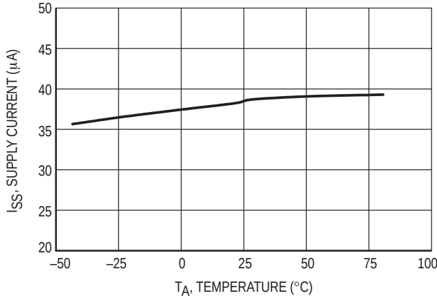
Figure 27. MC78PC50 Supply Current versus Temperature
