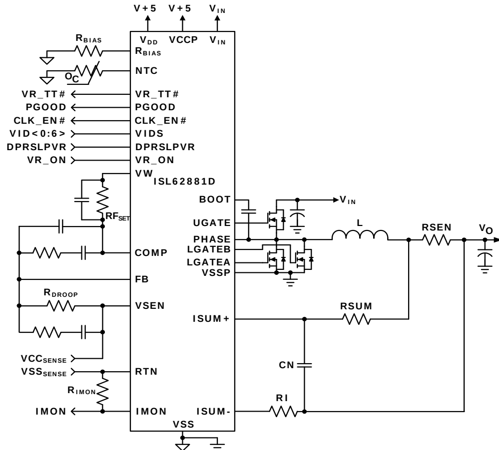
FIGURE 4. ISL62881D TYPICAL APPLICATION CIRCUIT USING RESISTOR SENSING
