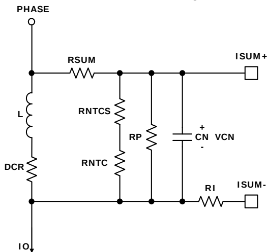
FIGURE 13. DCR CURRENT-SENSING NETWORK
