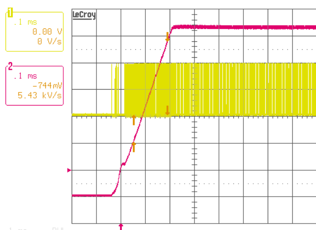
FIGURE 33. GPU MODE SOFT-START, V_{IN} = 19V , I_O = 0A , V_{ID} = 1.2V , Ch1: PHASE, Ch2: V_O
