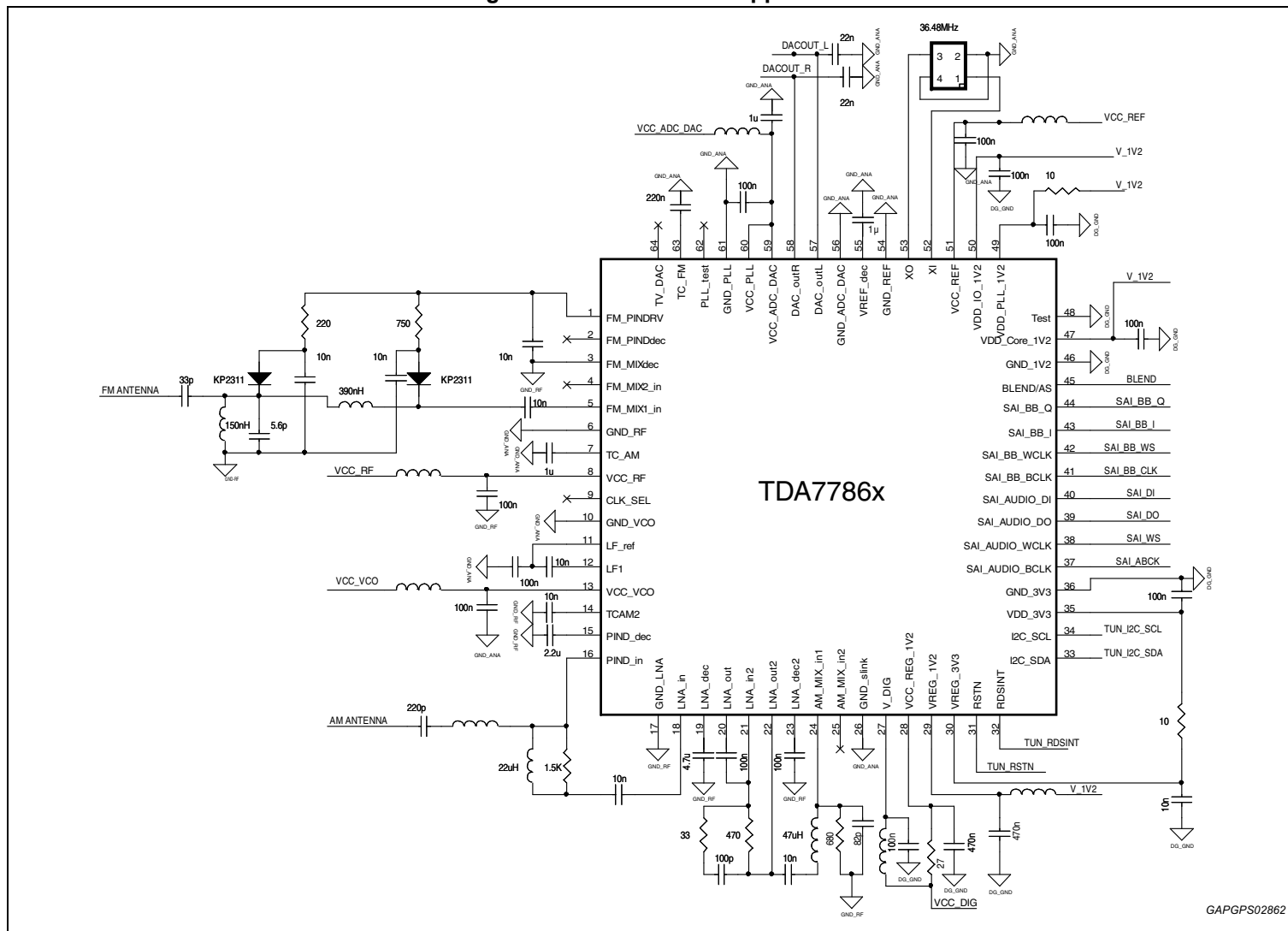
Figure 24. FM wide-band application
