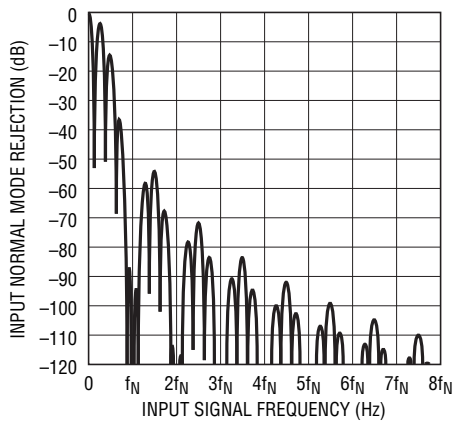
Figure 32. Input Normal Mode Rejection at DC
