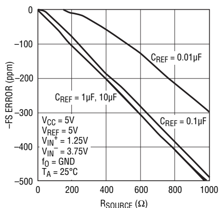
Figure 18. -FS Error vs R_{\text{SOURCE}} at V_{\text{REF}} (Large C_{\text{REF}} )
