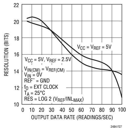
Figure 27. Resolution ( \text{INL}_{\text{RMS}} \leq 1\text{LSB} ) vs Output Data Rate and Reference Voltage
