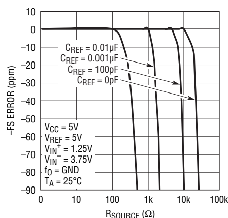
Figure 16. -FS Error vs R_{\text{SOURCE}} at V_{\text{REF}} (Small C_{\text{REF}} )
