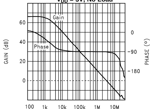
Open Loop Frequency Response V_{DD} = 3V , No Load
