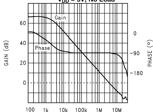
Open Loop Frequency Response V_{DD} = 5V , No Load
