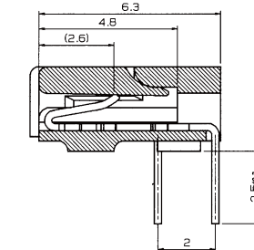
SECT. X-X
