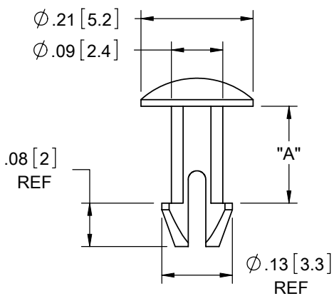
FIG 2. SLP-1-100 SERIES
