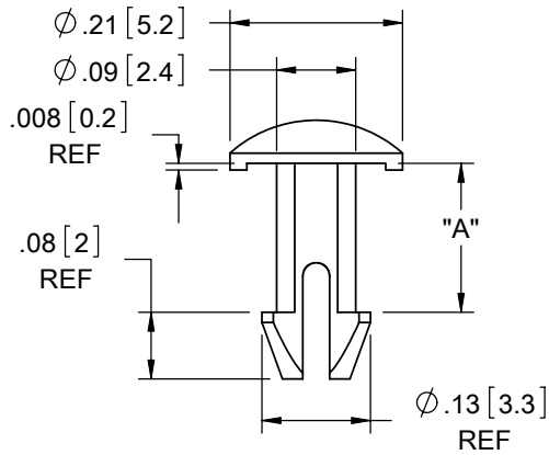
FIG 1. SLP100 SERIES
