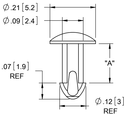
FIG 3. SLP-2-100 SERIES
