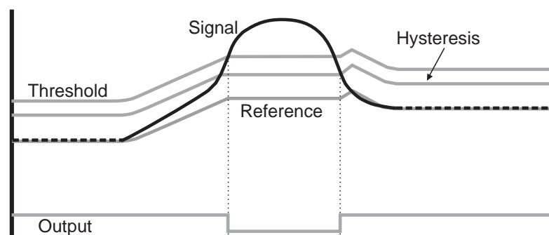
Figure 3-3. Drift Compensation
