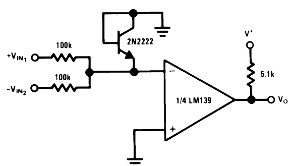
Figure 28. Basic Comparator
