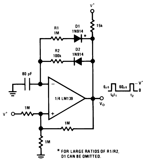
Figure 21. Pulse Generator
