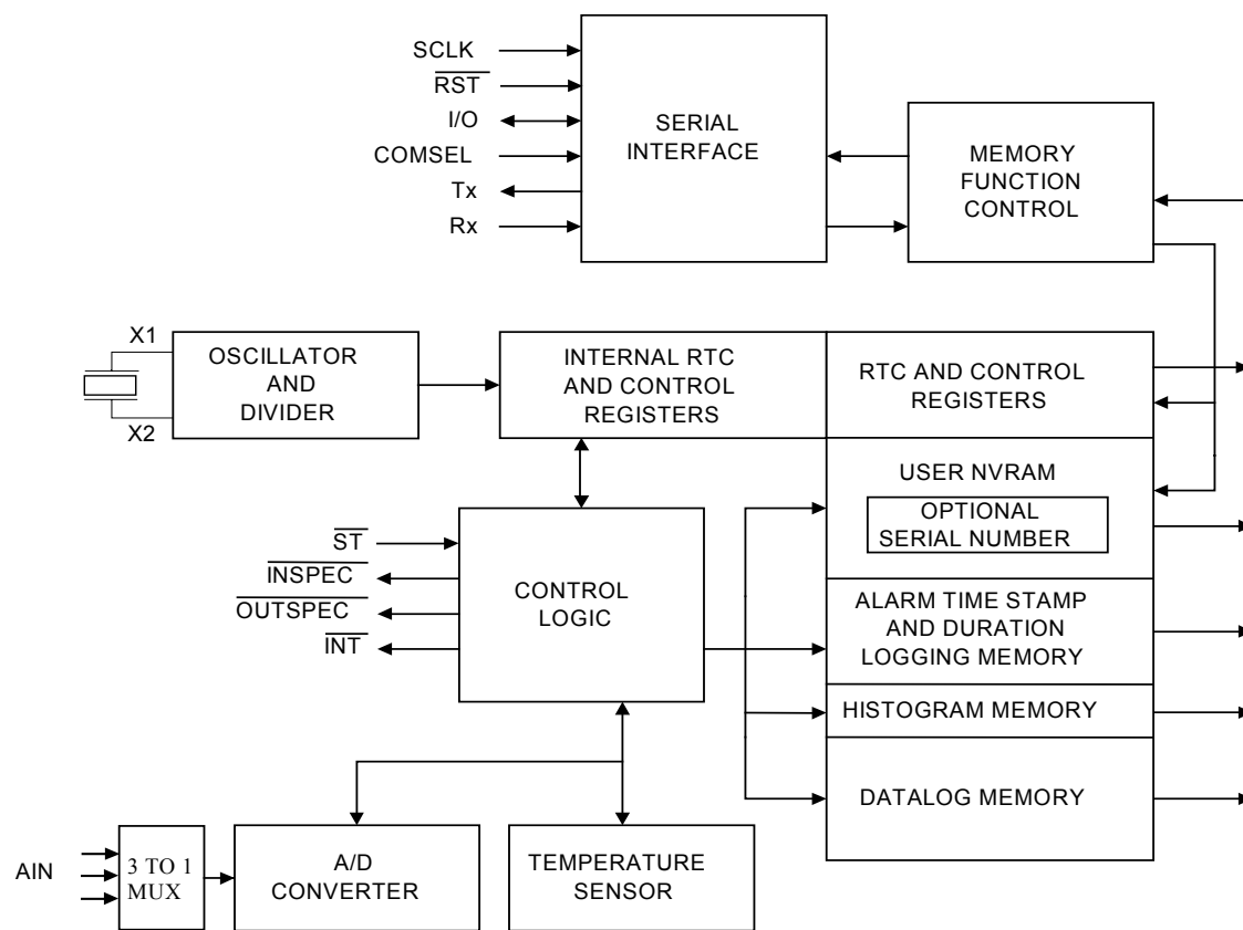
DS1616 Block Diagram Figure 1
