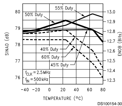
SINAD &amp; ENOB vs Clock Duty Cycle
