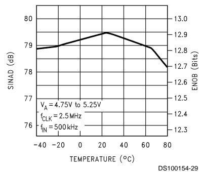
SINAD &amp; ENOB vs Temperature
