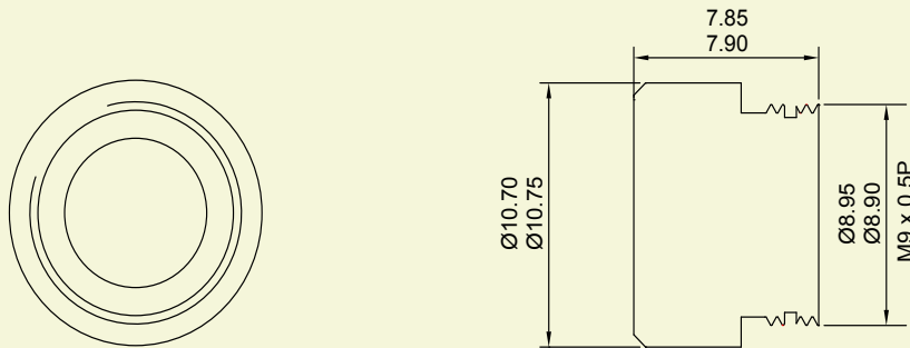
Interchangeable Line Lens (60° Fan Angle)
