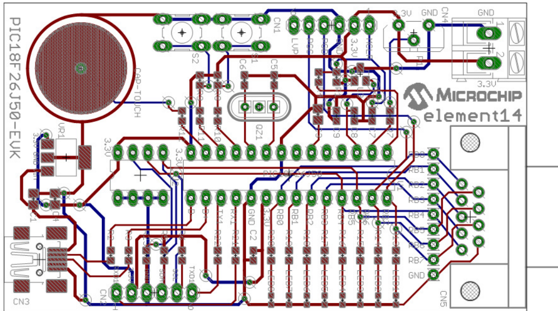
Figure 10–1 PCB Layout of PIC18F26J50-EVK
