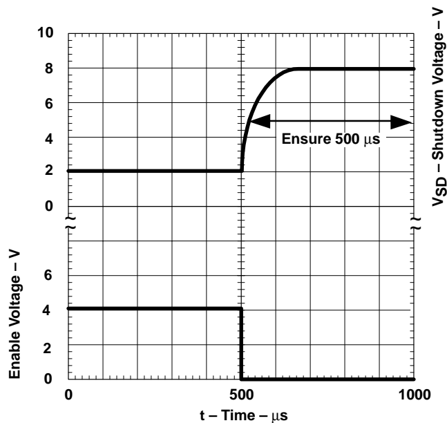
Figure 7. SD Timings
