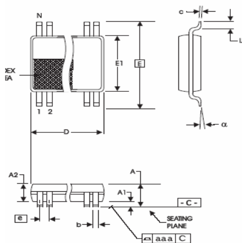
56 PIN TSSOP-240mil
