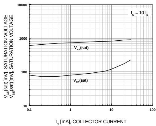
Figure 3. Saturation Voltage
