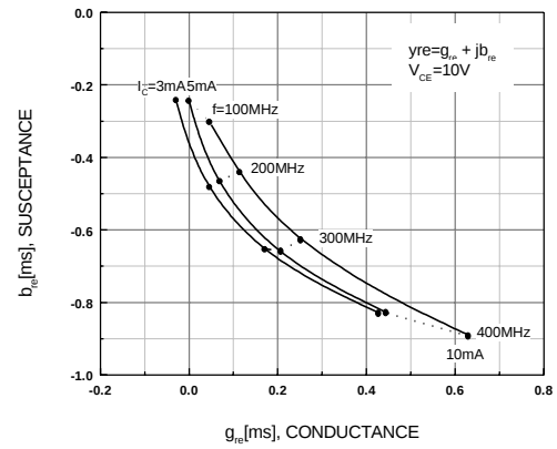
Figure 8. y_{re} - f
