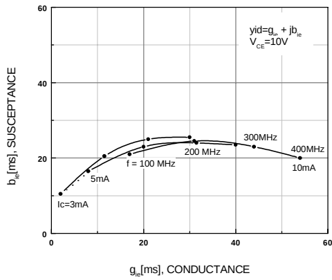
Figure 7. y_{id} - f
