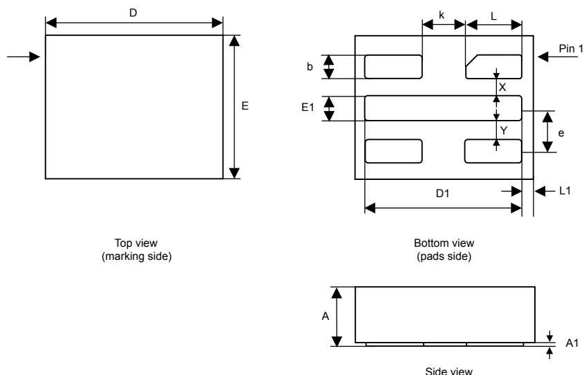
Figure 22. UFDFPN5 - Outline
