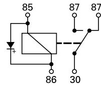
Change Over with Diode (C)
