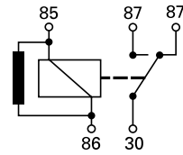
Change Over with resistor (B)
