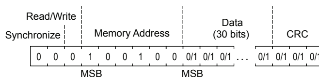
Figure 24: Access Code Write Sequence
