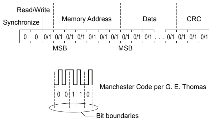
Figure 19: General Format for Serial Interface Commands
