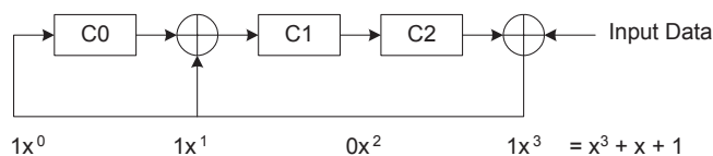
Figure 18: CRC Calculation
