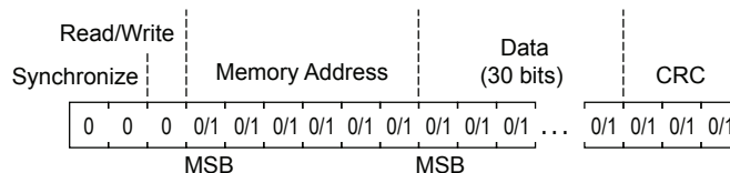
Figure 23: Write Sequence
