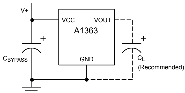
Figure 10: Typical Application Drawing
