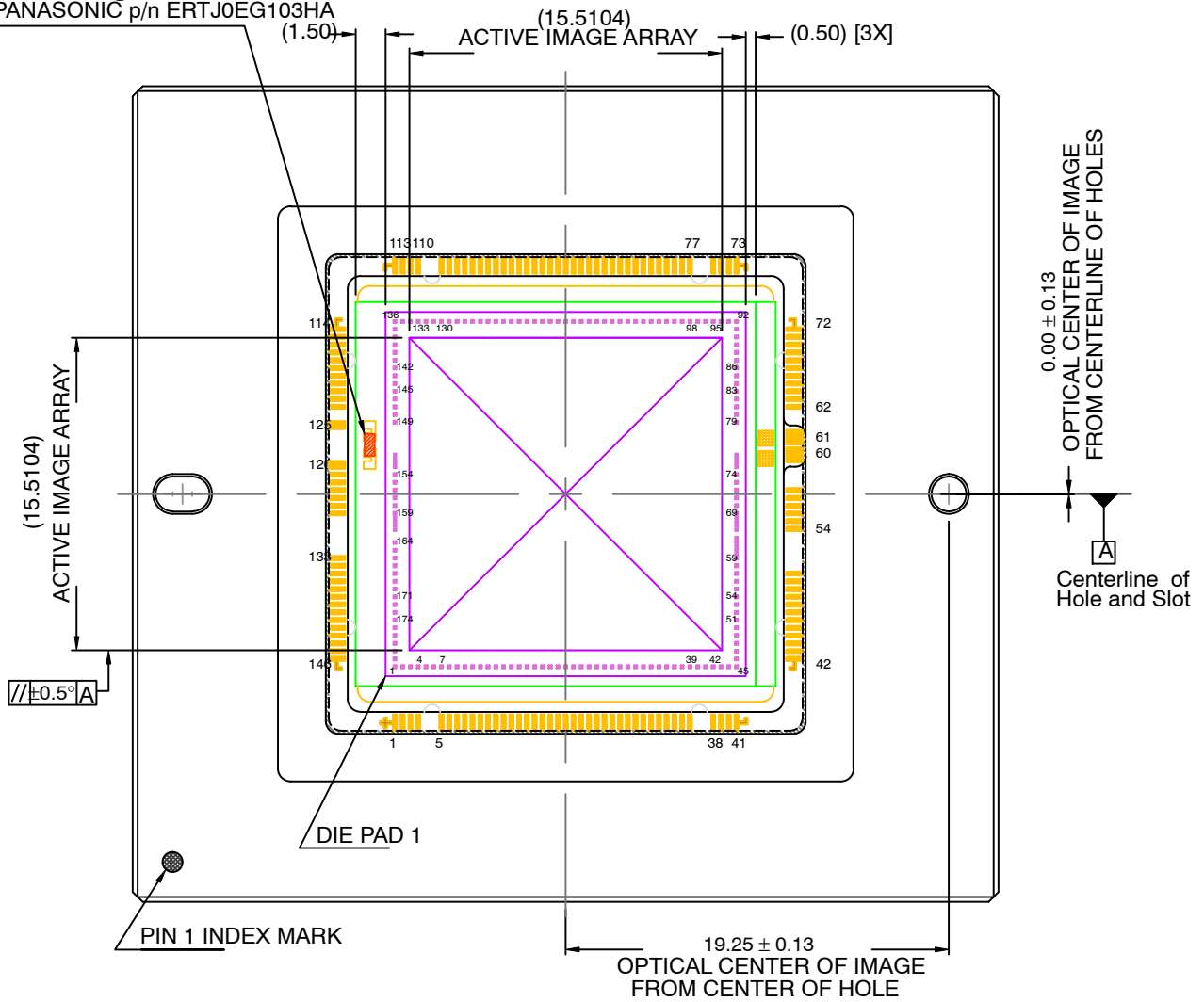
Figure 43. PGA Completed Assembly with Integrated TEC (4 of 4)
